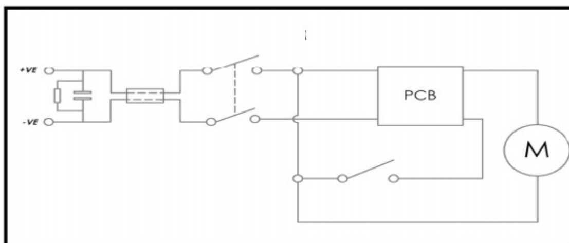
PVR - PVT Range (AUTOSAVE) Wiring Diagram
