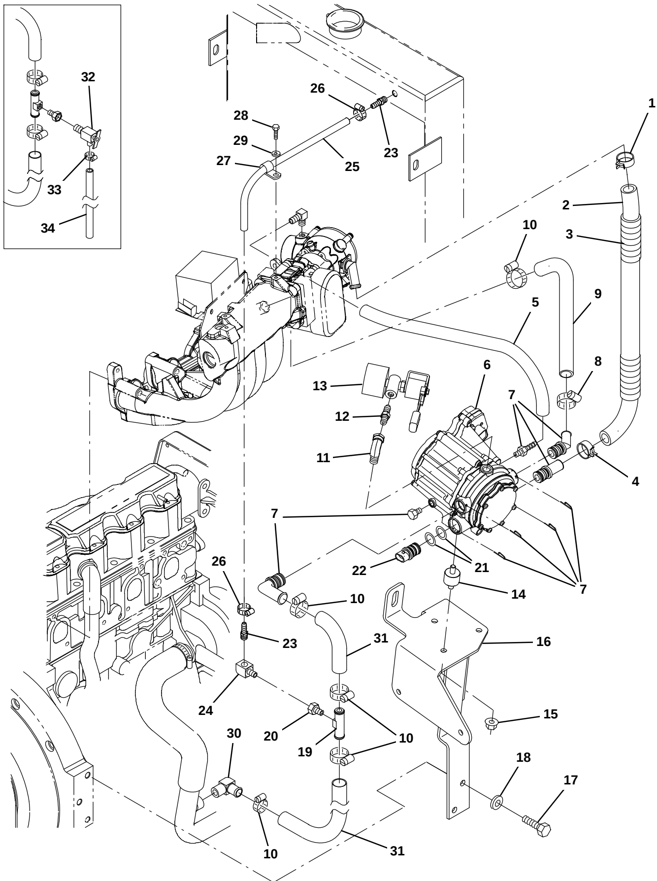
Fig. 17 – GM Engine Vaporizer Group, LPG (0047-0222)
