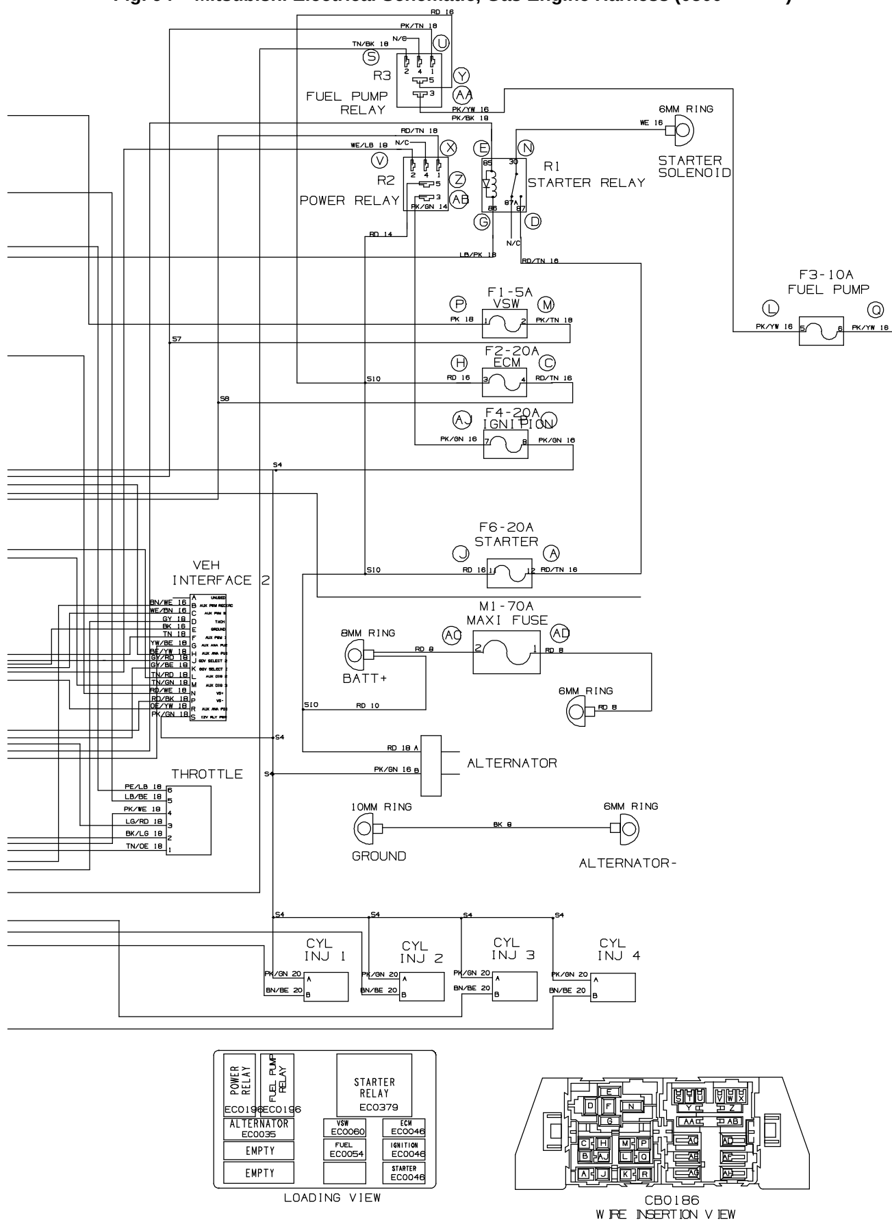
Fig. 94 – Mitsubishi Electrical Schematic, Gas Engine Harness (0500– )
