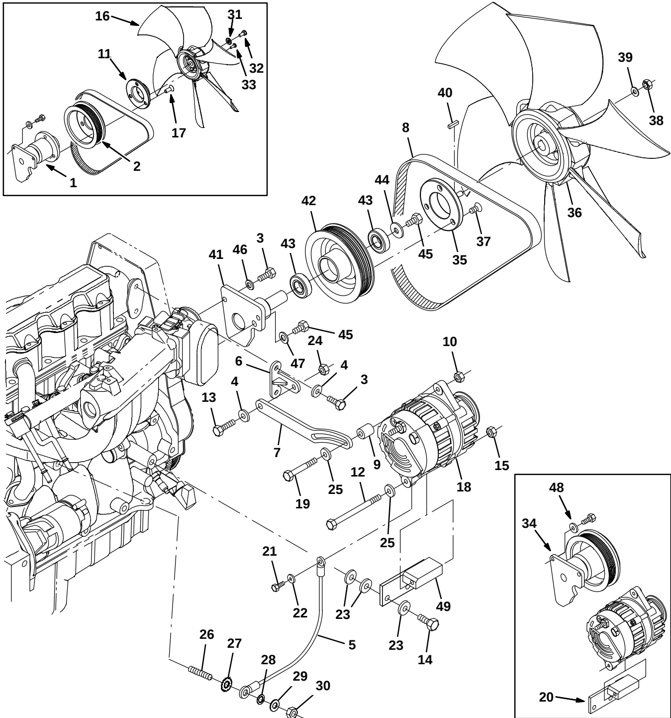
Fig. 24 – GM Engine Alternator and Fan Group (0000–0499)
