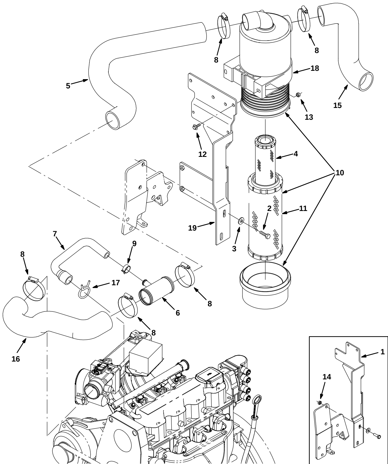
Fig. 21 – GM Engine Air Cleaner Group, Gasoline (0047–0499)
