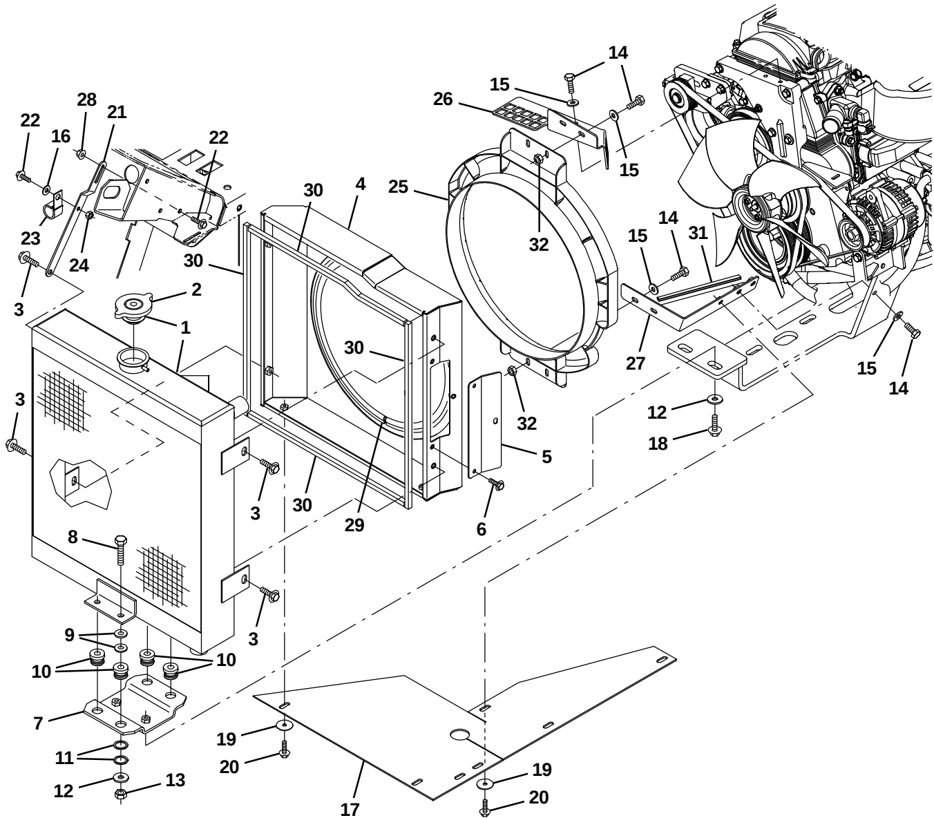
Fig. 38 – Mitsubishi Engine Radiator and Mount Group (0500– )
