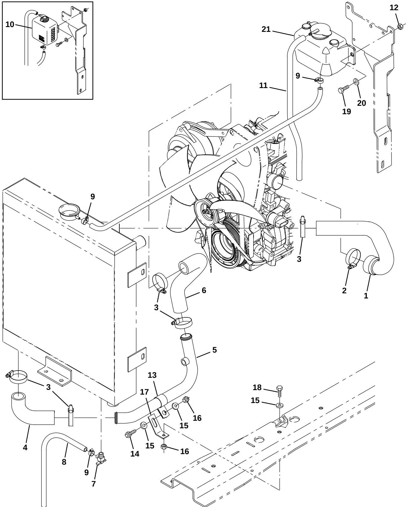
Fig. 29 – GM Engine Radiator Hose Group (0196–0499)
