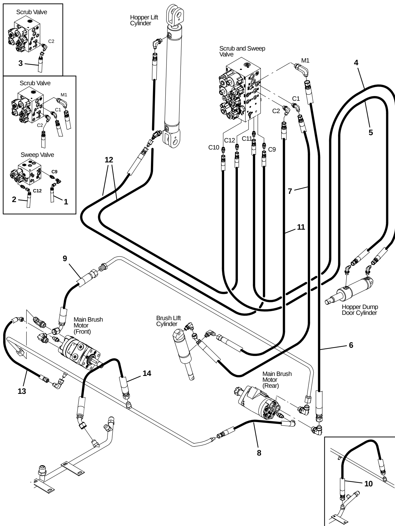
Fig. 77 – Hydraulic Hose Group, Brush and Hopper
