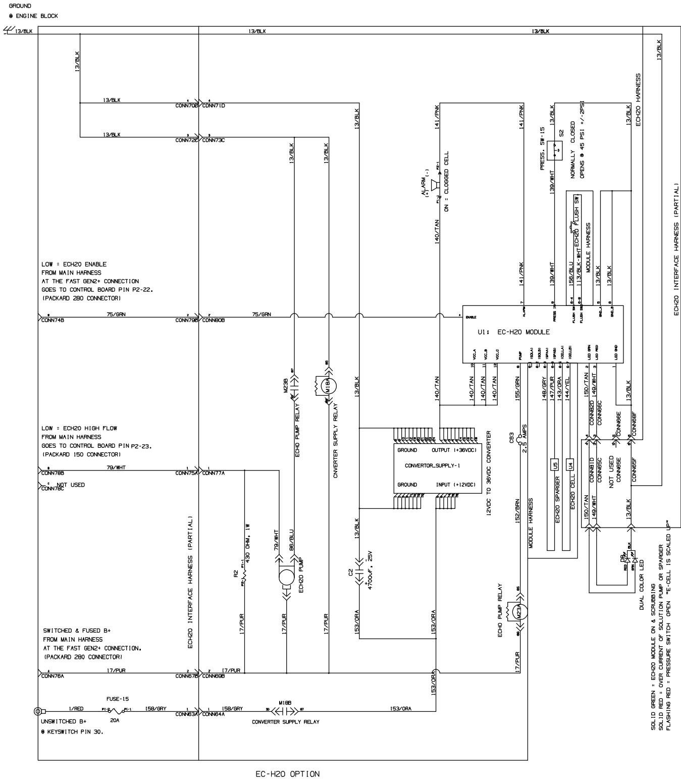
Fig. 86 – GM Electrical Schematic (0145-xxxx)
