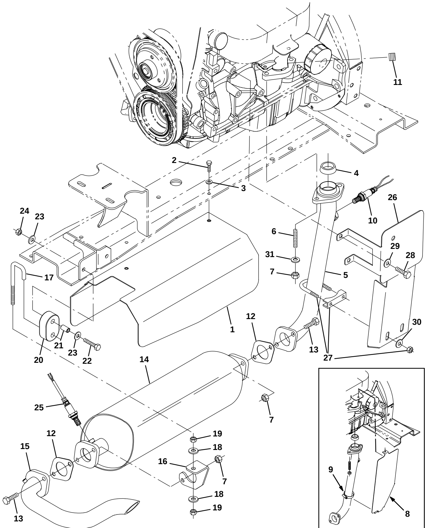
Fig. 26 – GM Engine Muffler Group (0047–0499)
