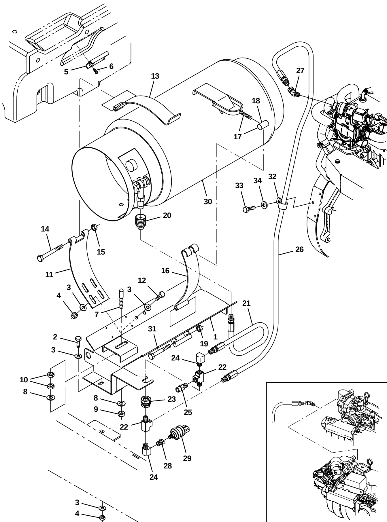
Fig. 41 – Engine Fuel Tank Group, LPG
