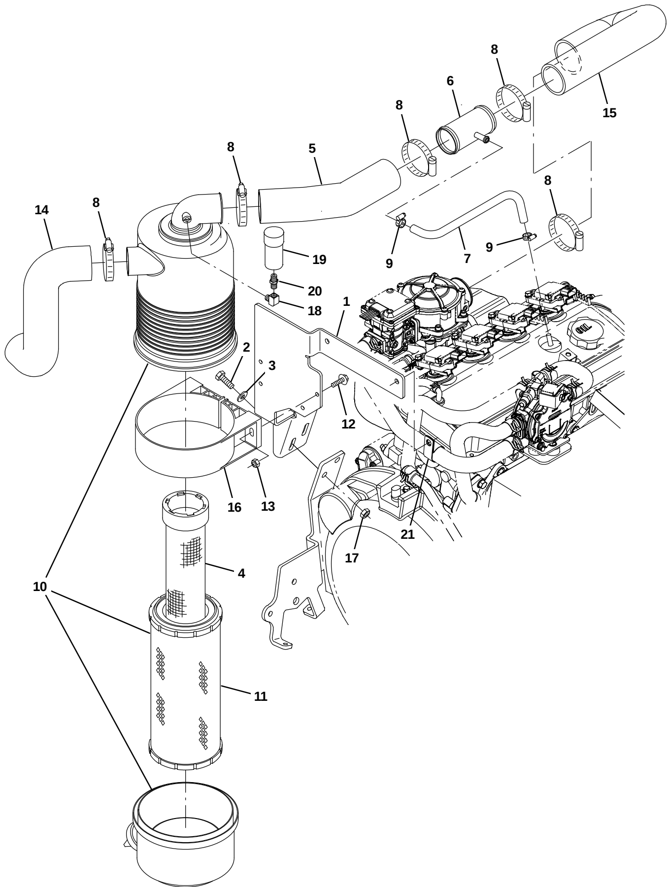
Fig. 35 – Mitsubishi Engine Air Cleaner Group, LPG (0500– )
