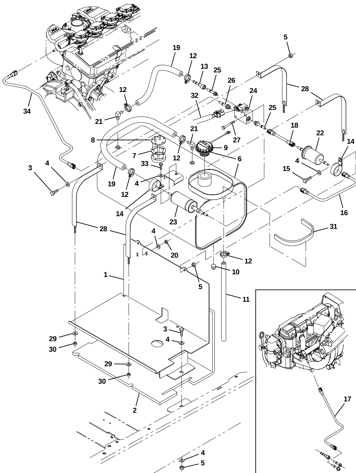
Fig. 40 – Engine Fuel Tank Group, Gasoline (0047– )
