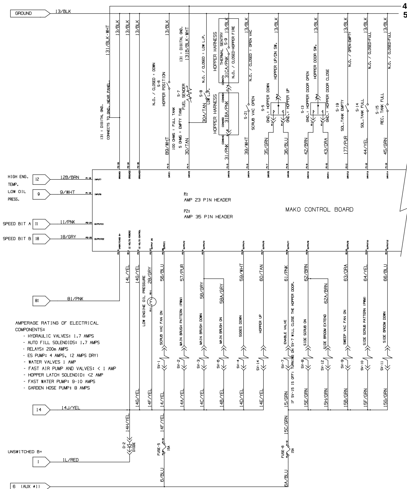
Fig. 85 – GM Electrical Schematic (0047-0145)
