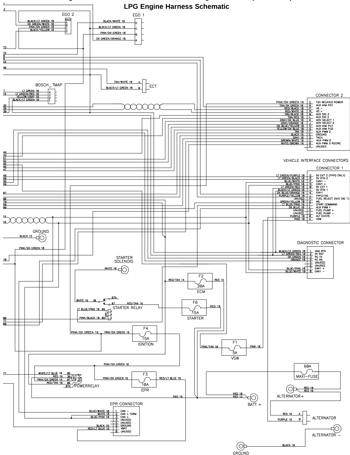
Fig. 91 – GM Electrical Schematic, LPG Engine Harness (0047–0222)
