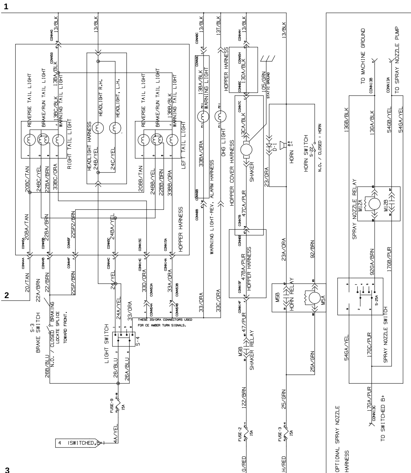
Fig. 85 – GM Electrical Schematic (0047-0145)
