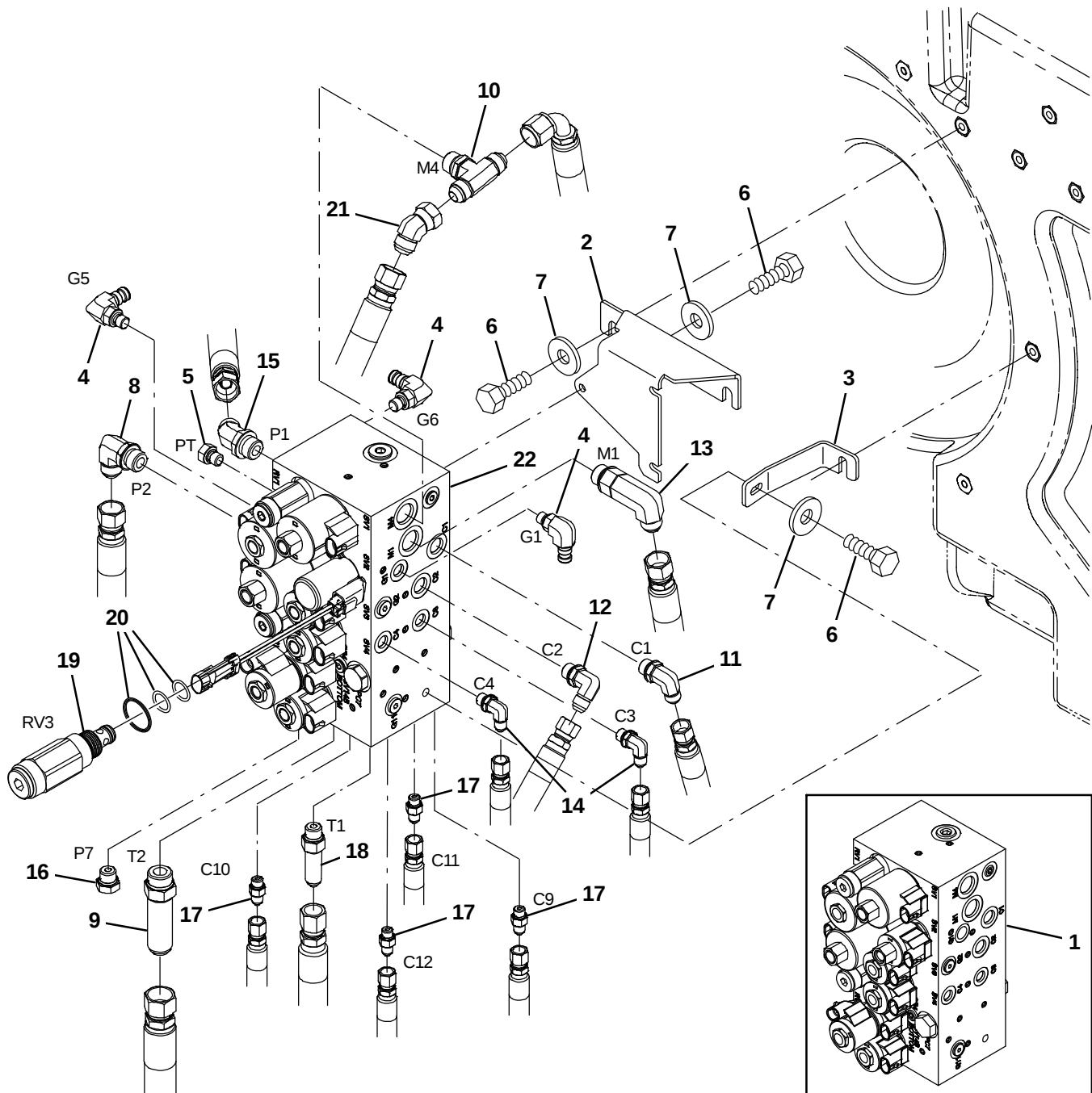
Fig. 83 – Hydraulic Valve Group (0132– )
