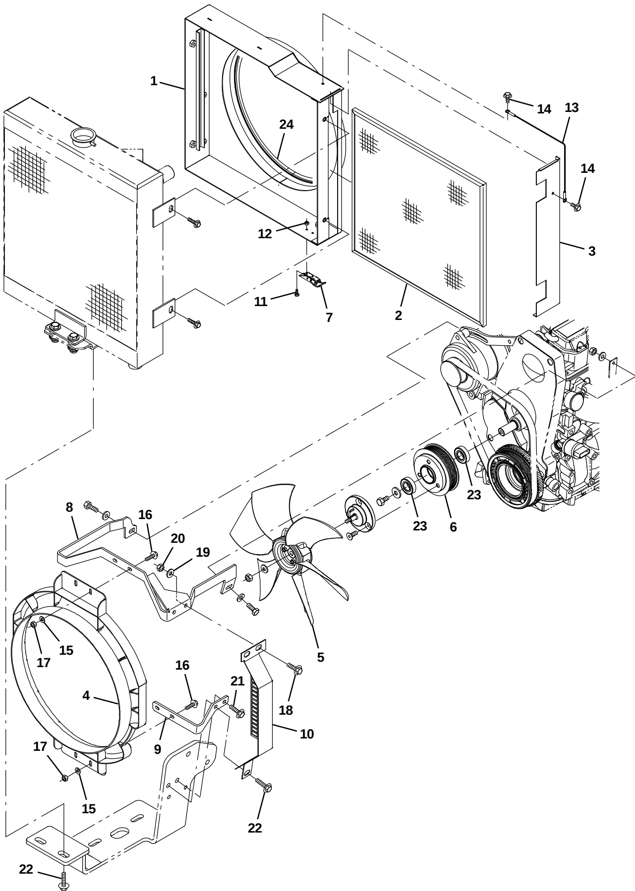
Fig. 29 – Engine Radiator Screen Kit (0196–0499)
