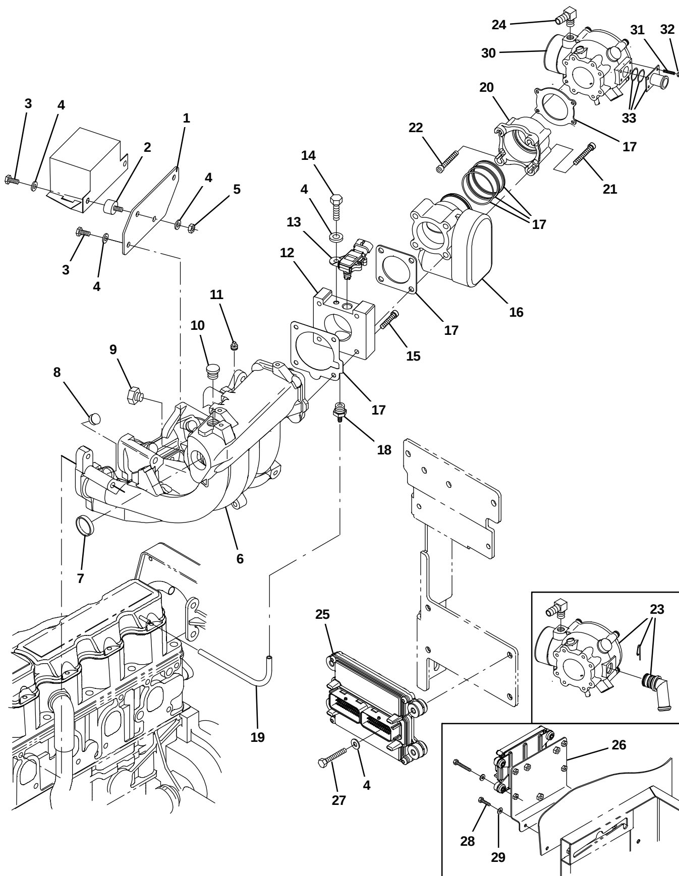
Fig. 16 – GM Engine EFI Group, LPG (0047–0499)
