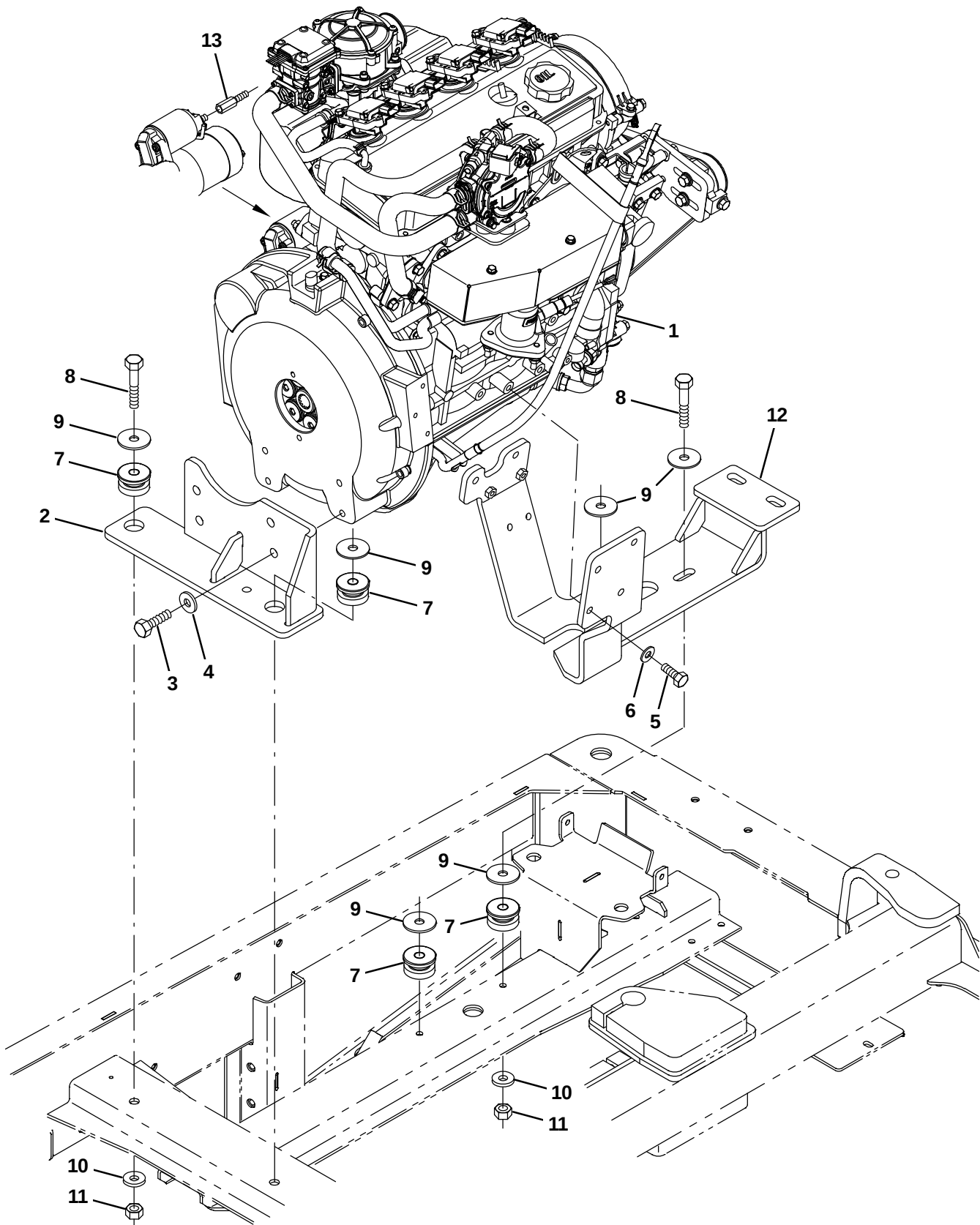
Fig. 31 – Mitsubishi Engine and Mount Group, LPG (0500– )
