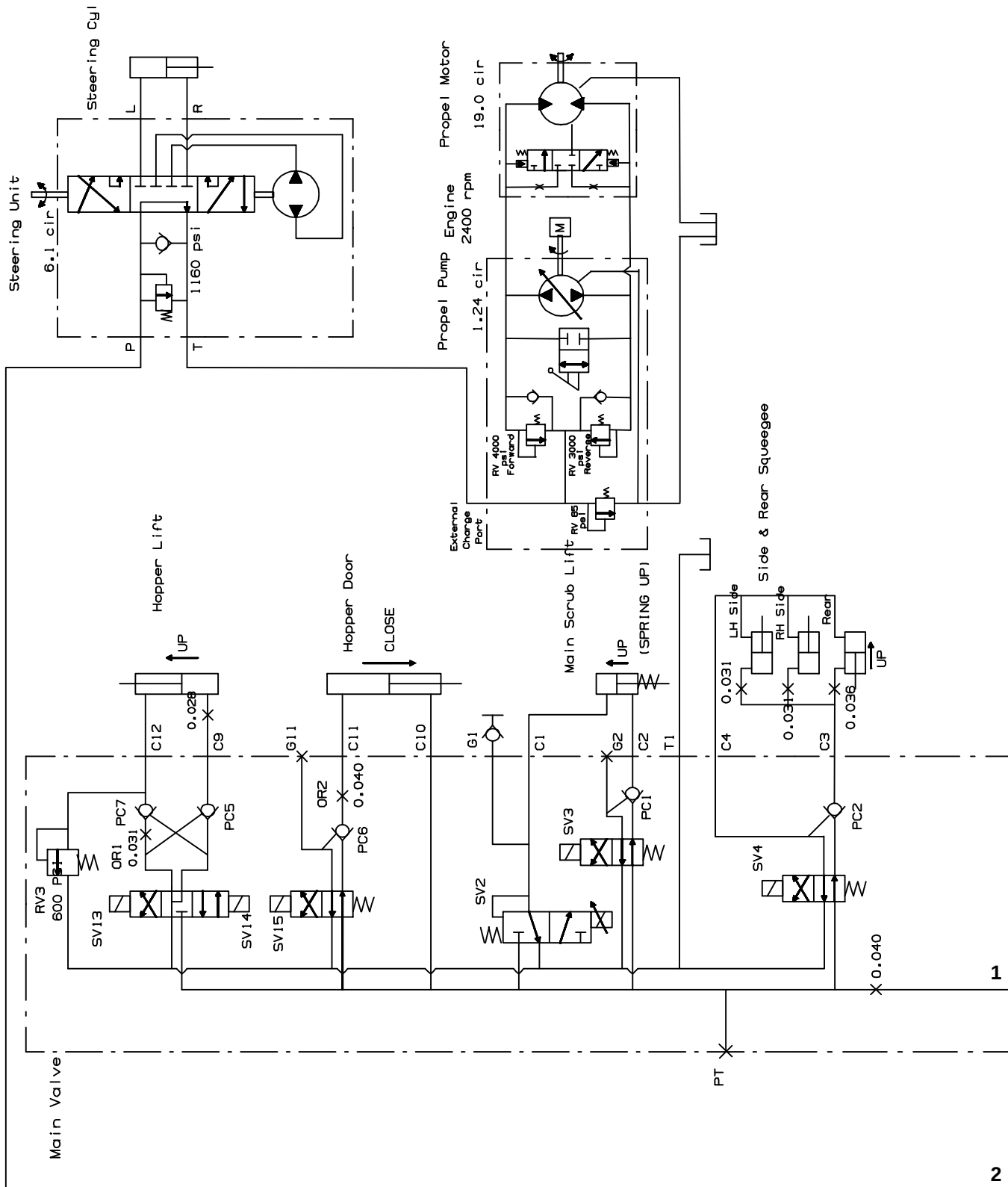
Fig. 73 – Hydraulic Schematic (0132–0270)
