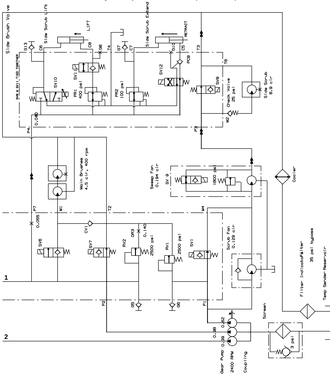
Fig. 74 – Hydraulic Schematic (0271– )
