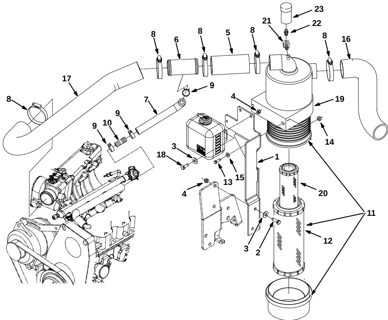
Fig. 20 – GM Engine Air Cleaner Group, Gasoline (0000–0046)
