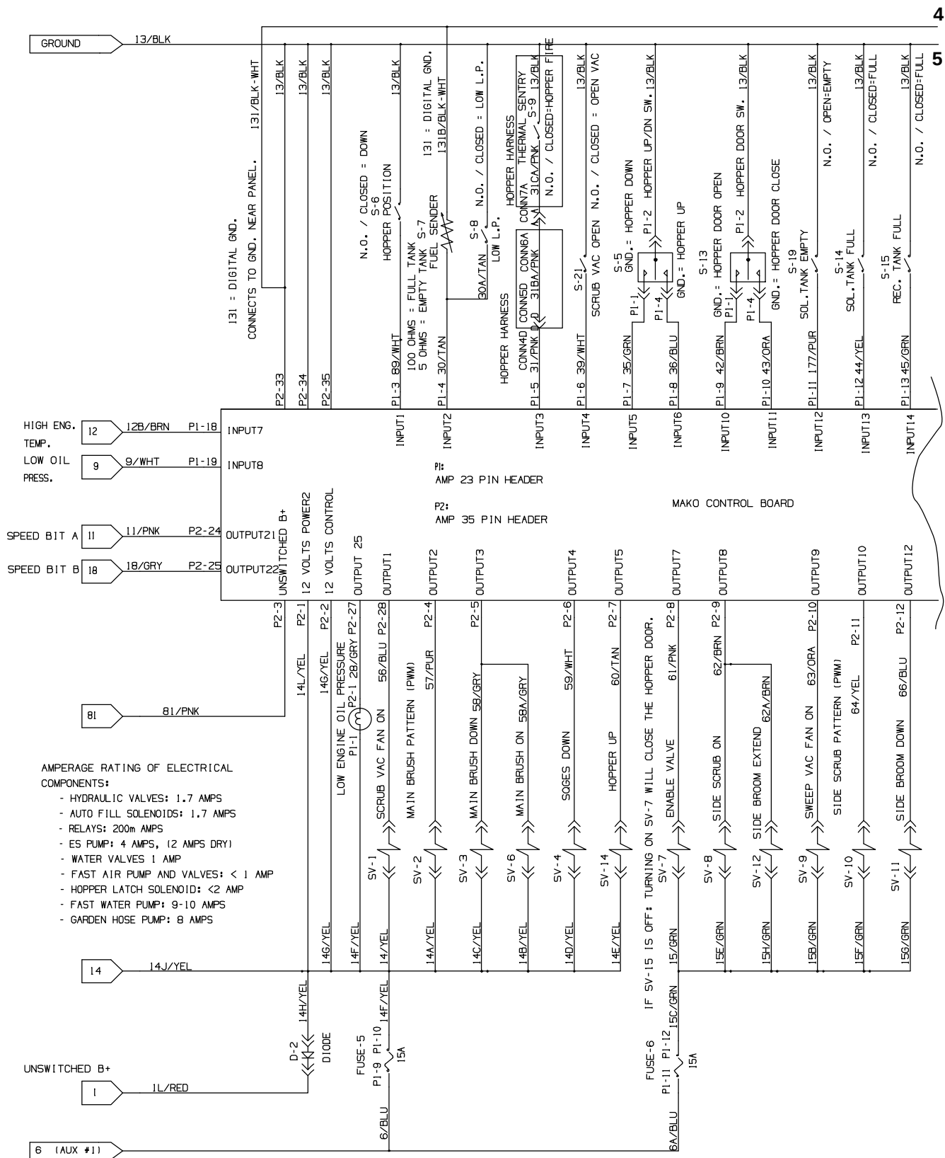
Fig. 84 – GM Electrical Schematic (0000–0046)
