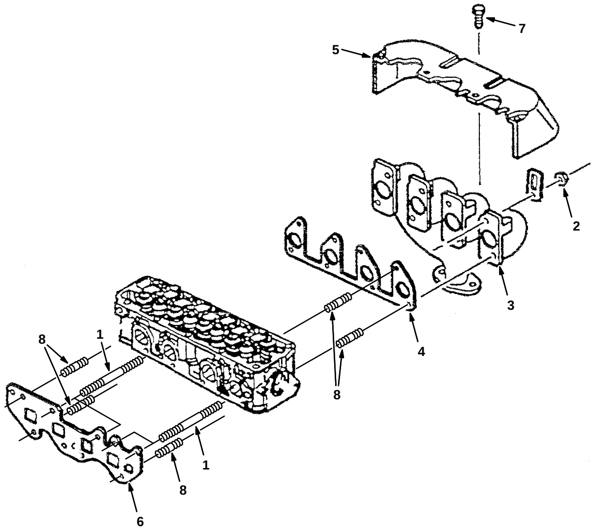
Fig. 5 – Manifold Group
