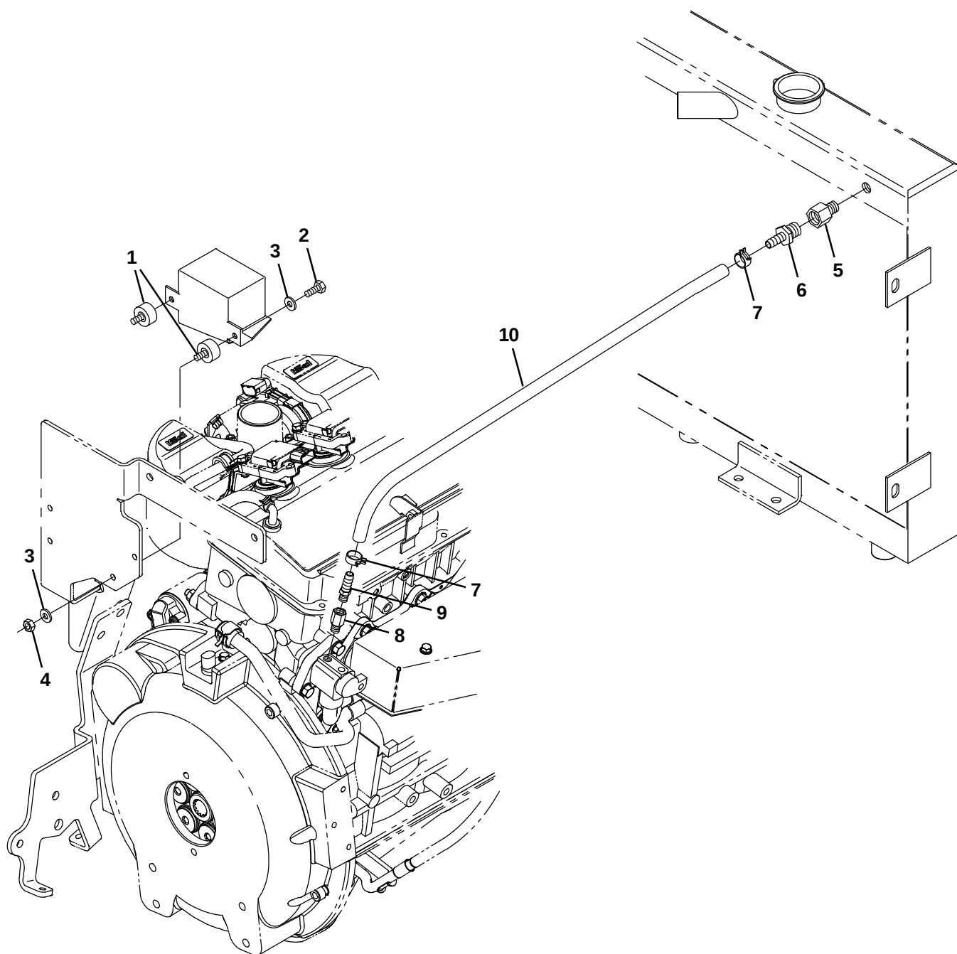
Fig. 32 – Mitsubishi Engine EFI Group, Gasoline (0500– )
