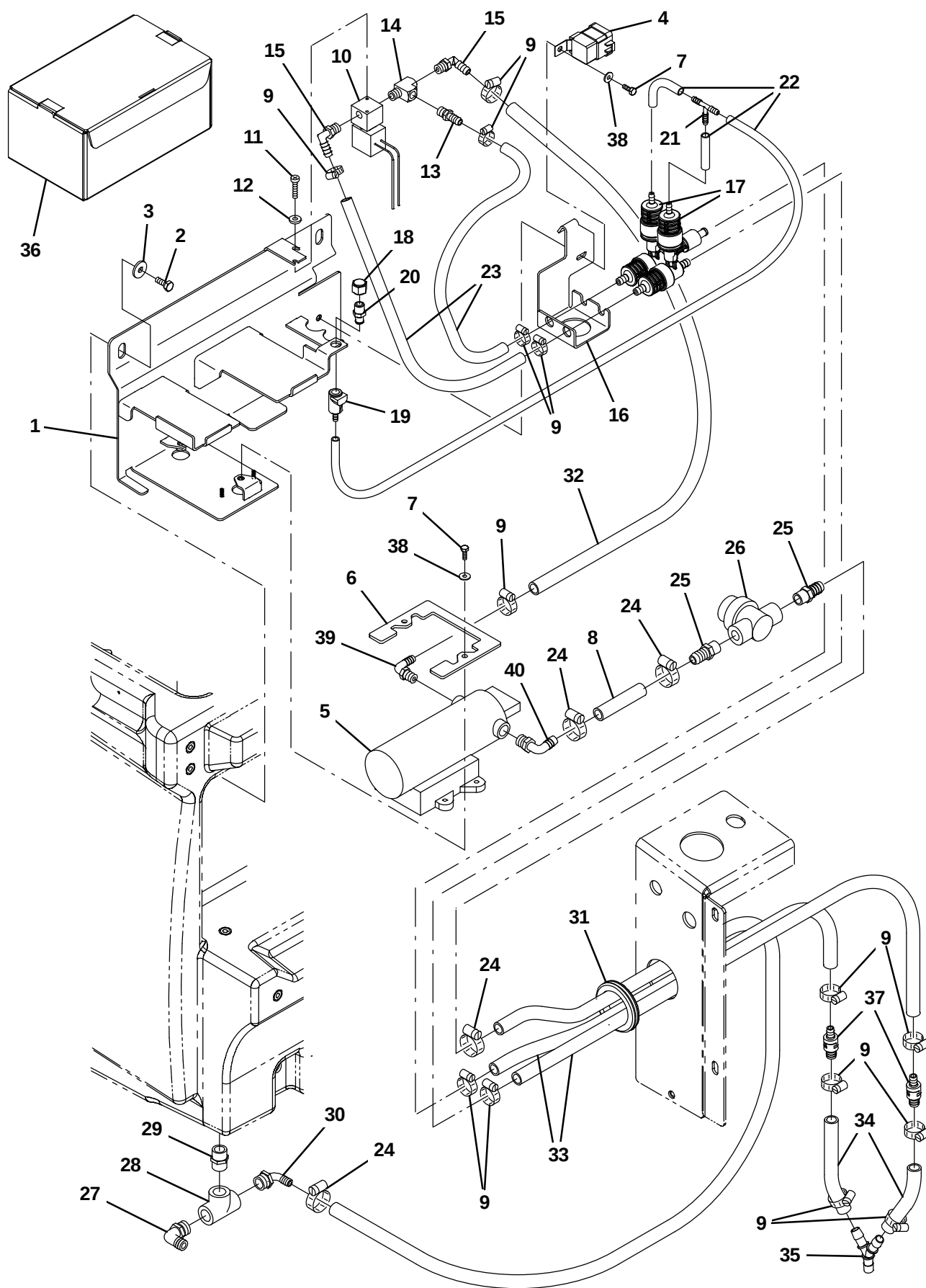
Fig. 14 – FaST Pumps and Detergent Group (0146– )
