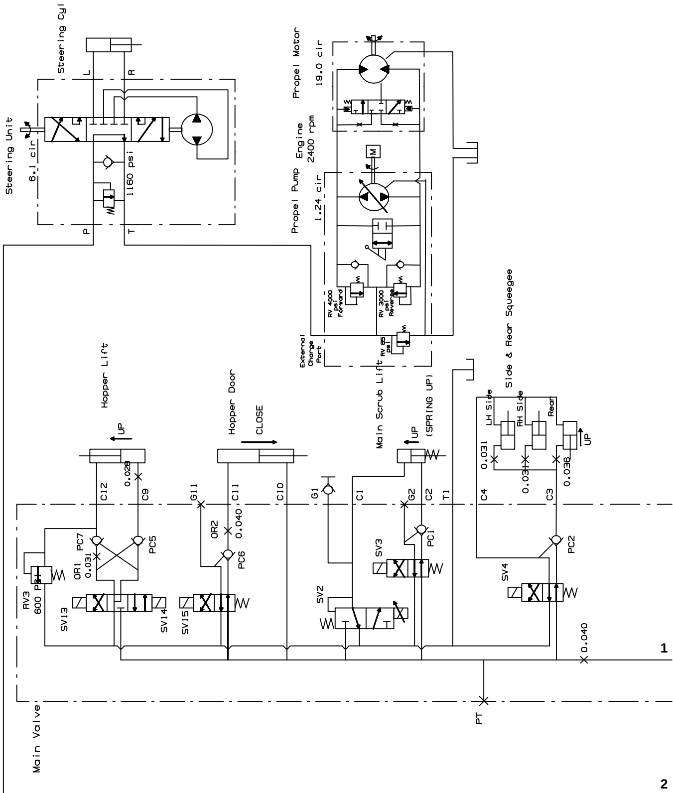
Fig. 74 – Hydraulic Schematic (0271- )
