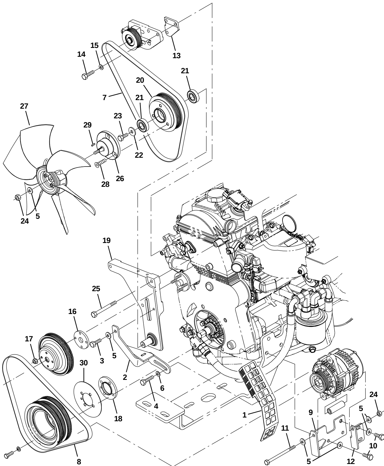
Fig. 36 – Mitsubishi Engine Alternator and Fan Group (0500– )
