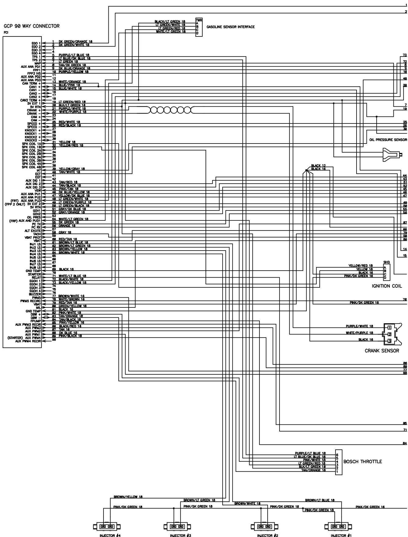
Fig. 90 – GM Electrical Schematic, Gas Engine Harness (0223-0499)
