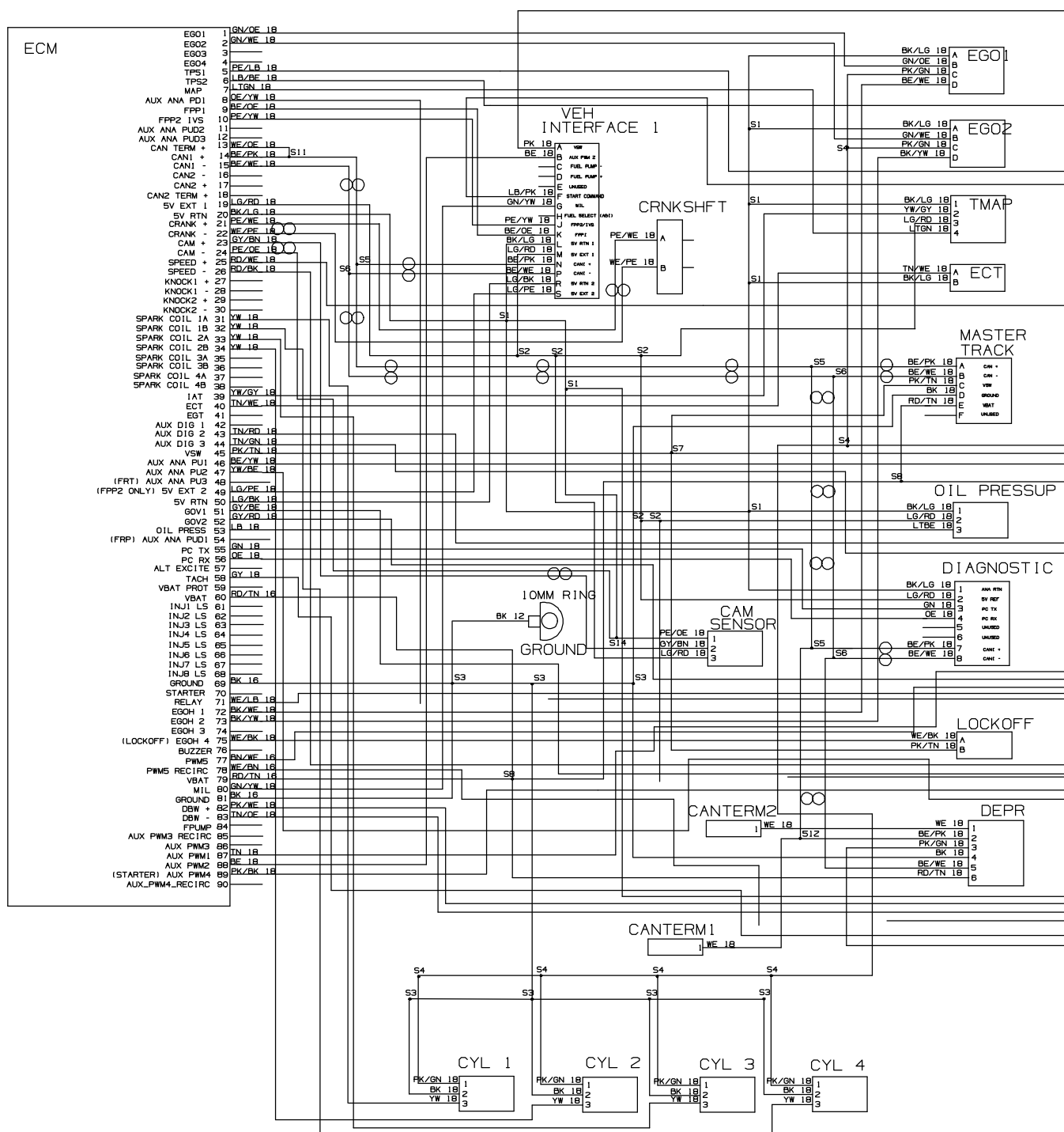
Fig. 95 – Mitsubishi Electrical Schematic, LPG Engine Harness (0500– )
