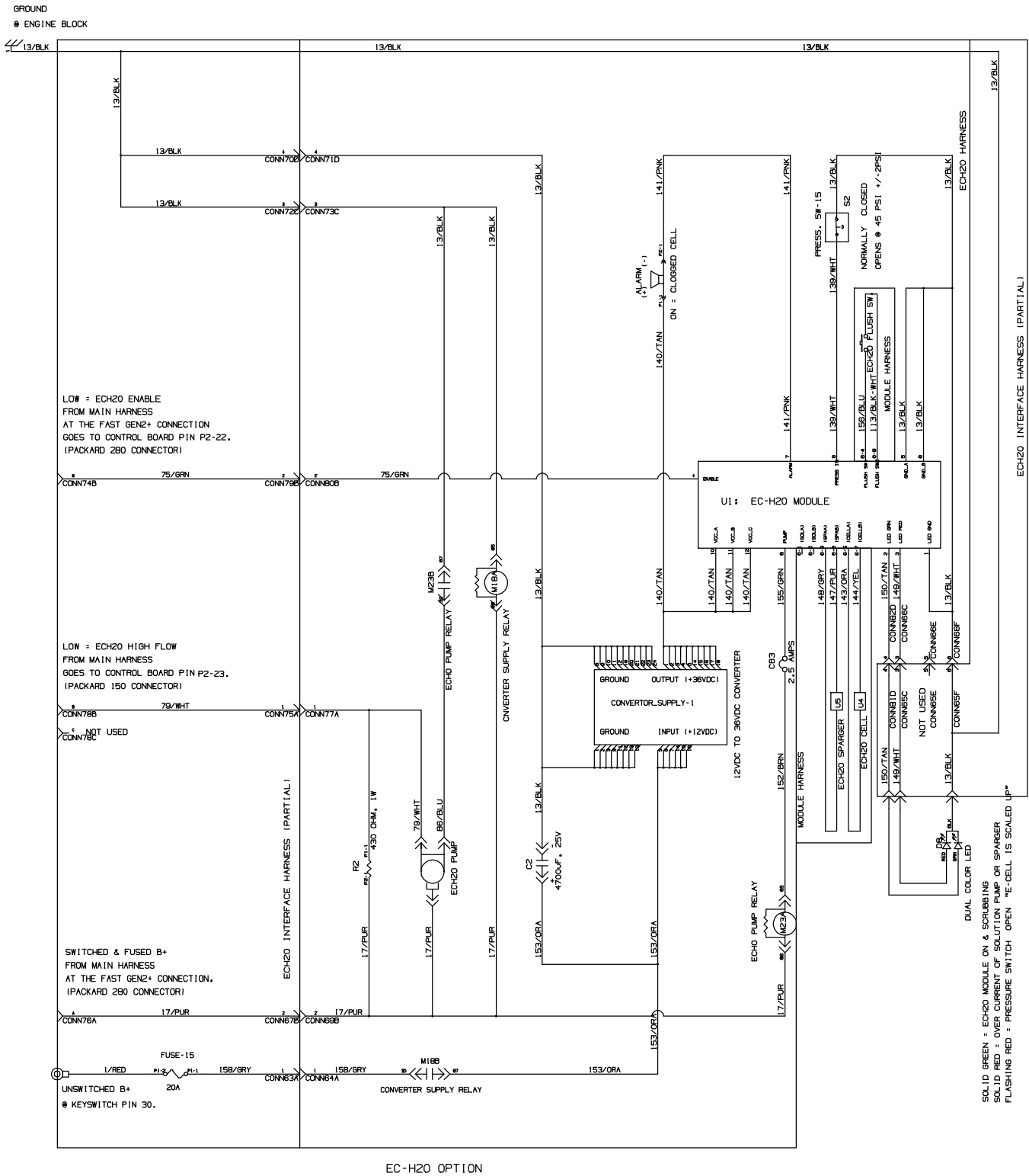
Fig. 87 – GM Electrical Schematic (xxxx-0499)
