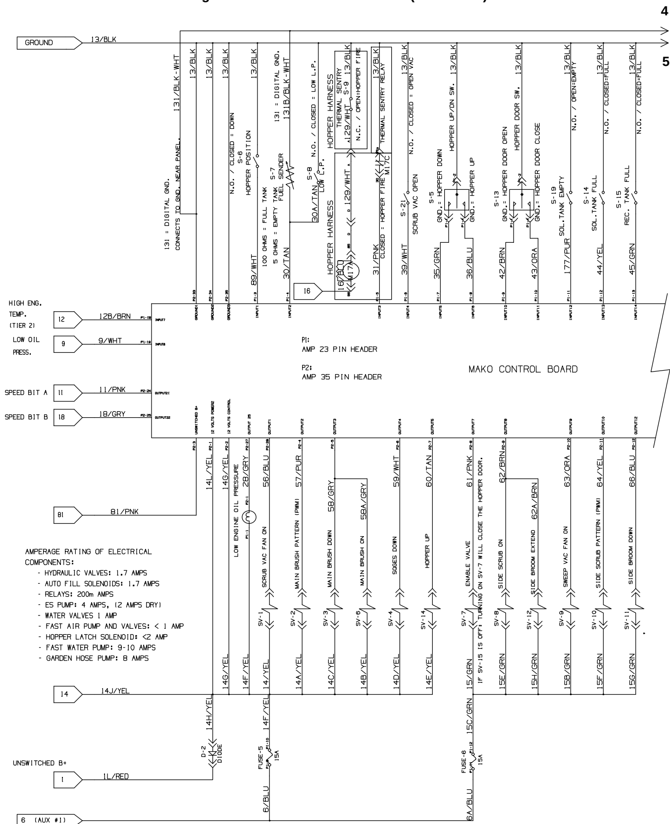
Fig. 87 – GM Electrical Schematic (xxxx-0499)
