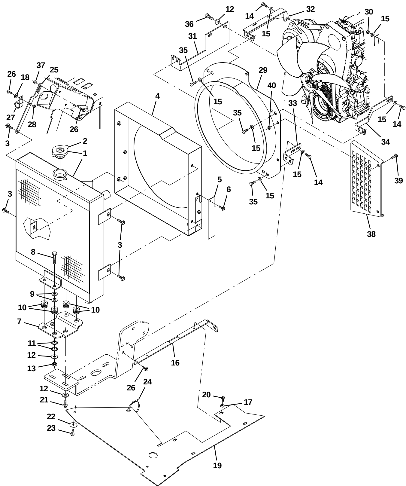
Fig. 28 – GM Engine Radiator and Mount Group (0196–0499)
