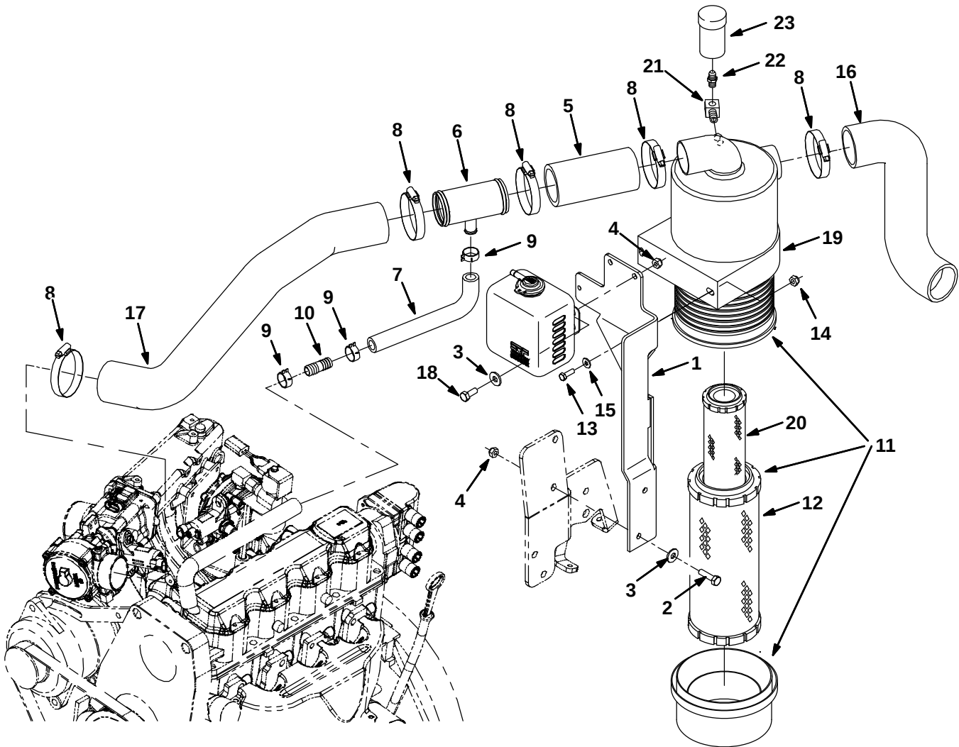
Fig. 22 – GM Engine Air Cleaner Group, LPG (0000–0046)
