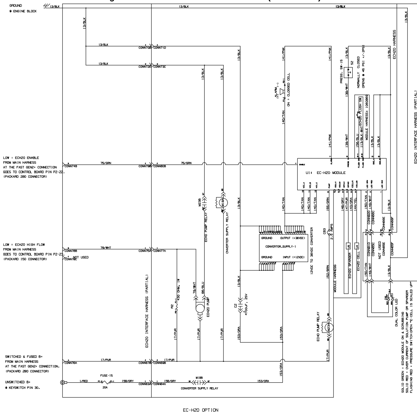
Fig. 93 – Mitsubishi Electrical Schematic (0500– )
