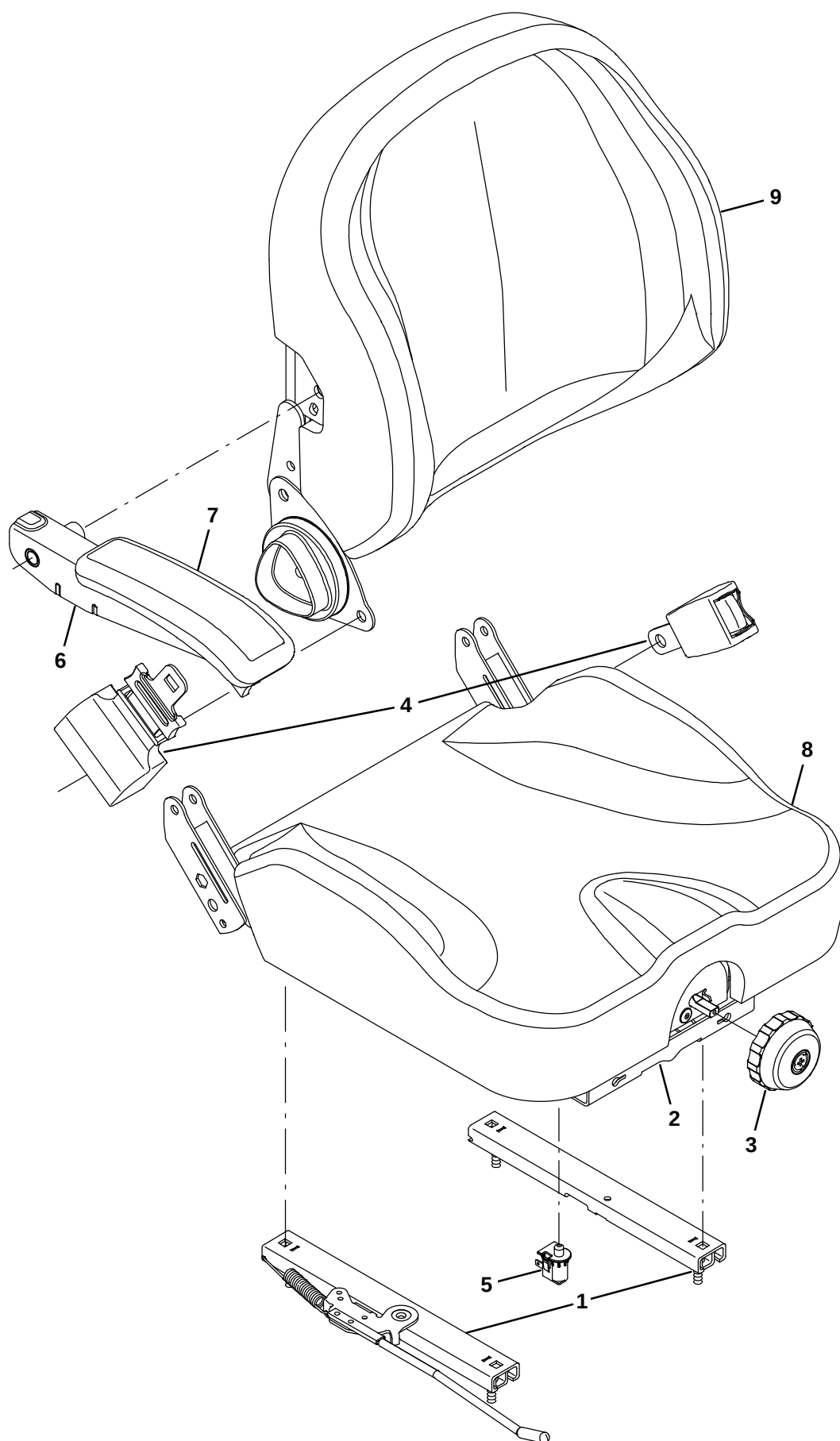
Fig. 18 – Seat Breakdown, 1072456
