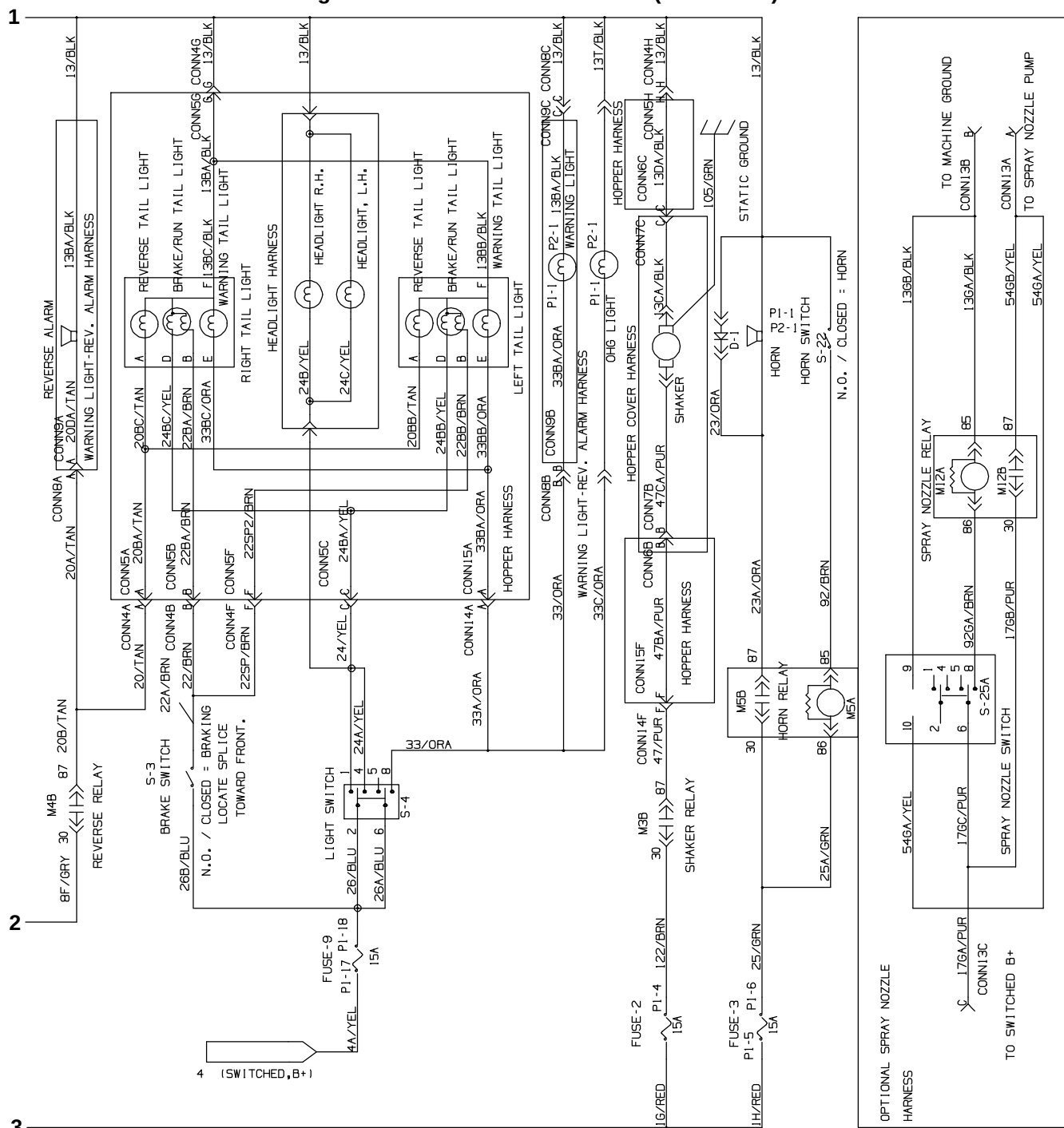
Fig. 84 – GM Electrical Schematic (0000-0046)
