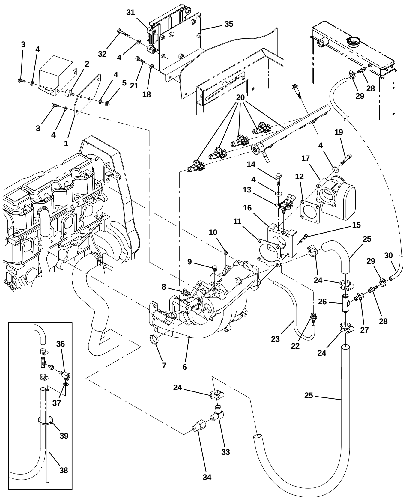
Fig. 13 – GM Engine EFI Group, Gasoline (0047-0222)
