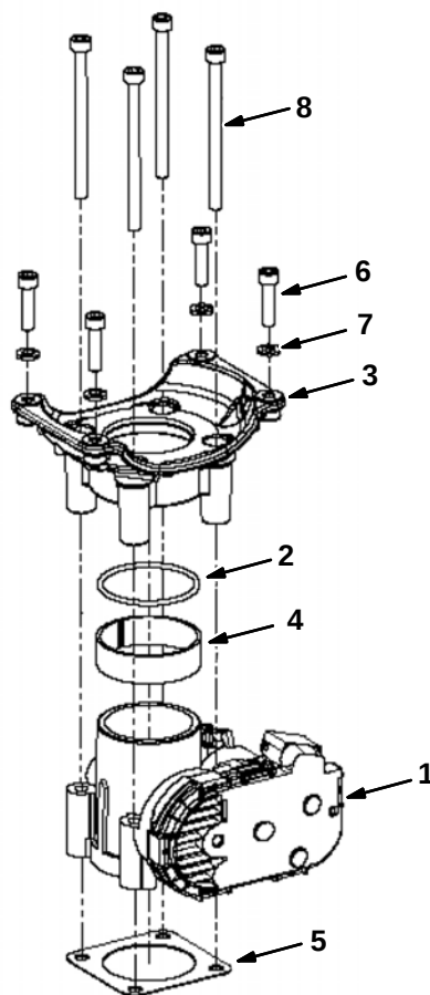
Fig. 22 – Throttle Body Group, LPG Engine
