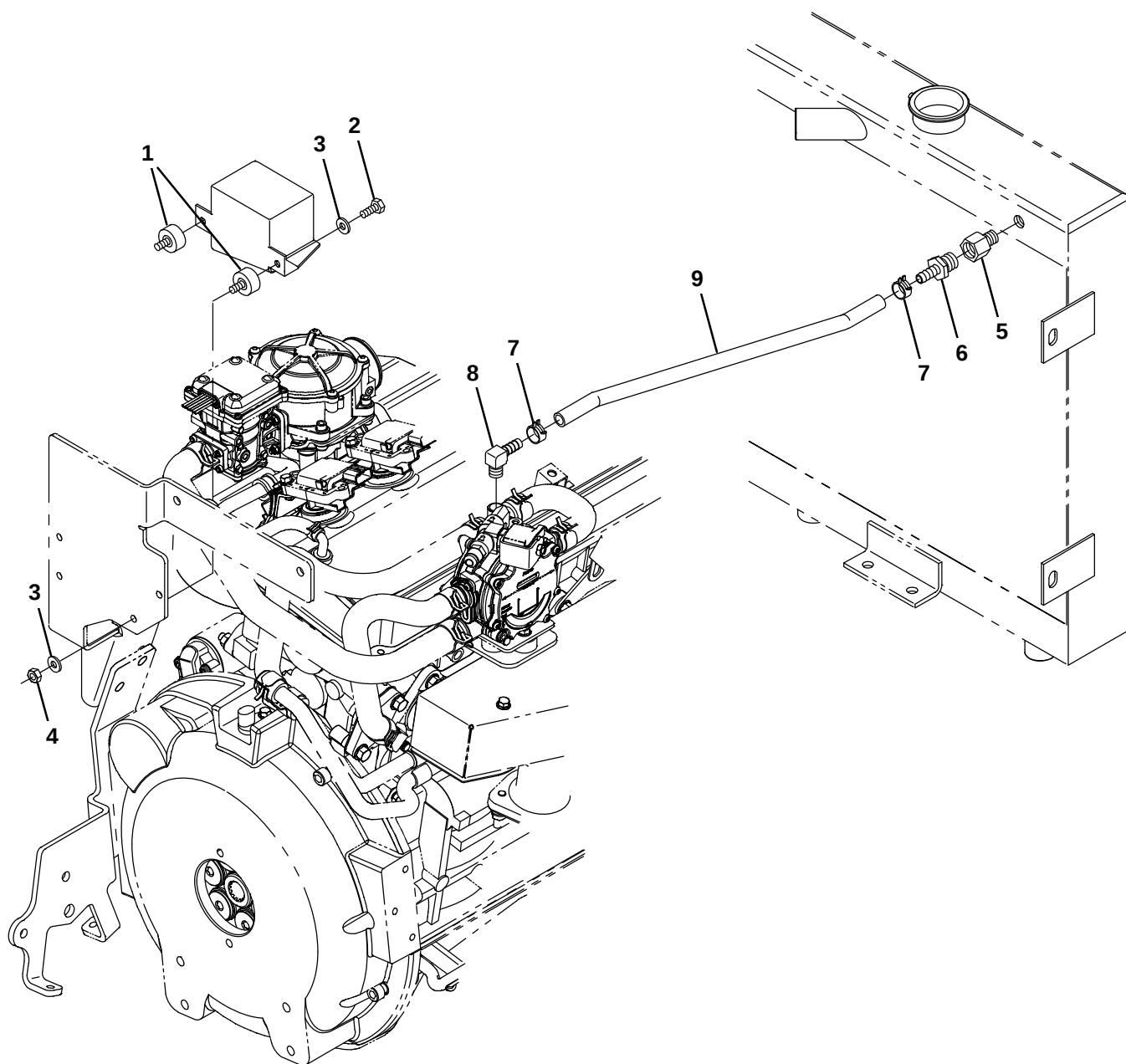
Fig. 33 – Mitsubishi Engine EFI Group, LPG (0500– )
