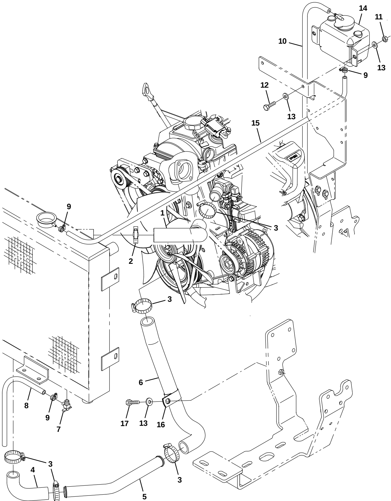
Fig. 39 – Mitsubishi Engine Radiator Hose Group (0500– )
