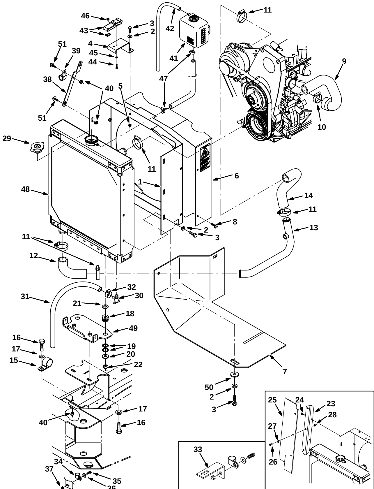
Fig. 27 – GM Engine Radiator Group (0000-0195)
