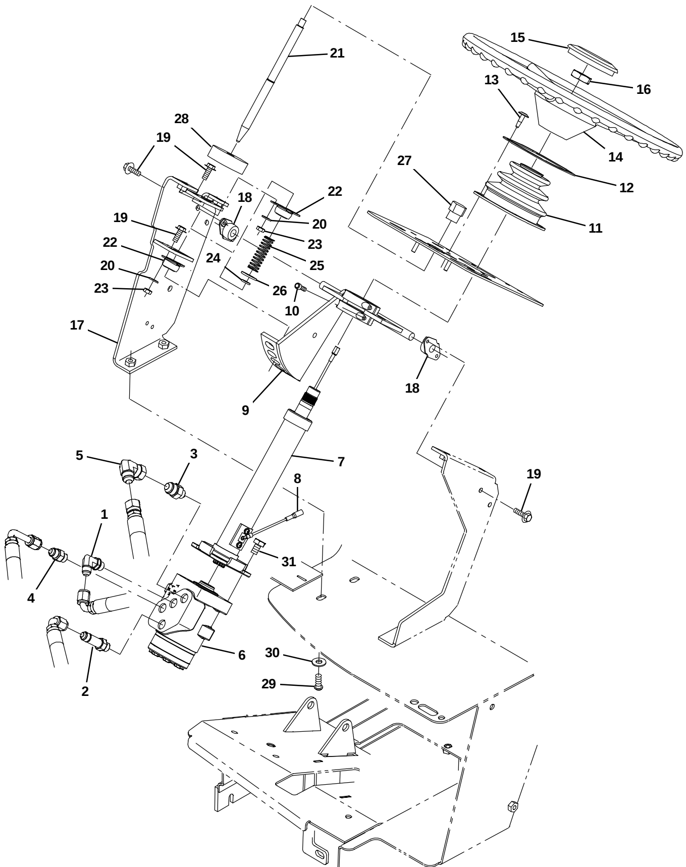
Fig. 8 – Steering Group
