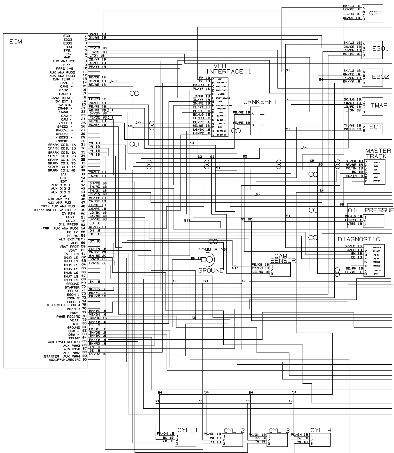
Fig. 94 – Mitsubishi Electrical Schematic, Gas Engine Harness (0500- )
