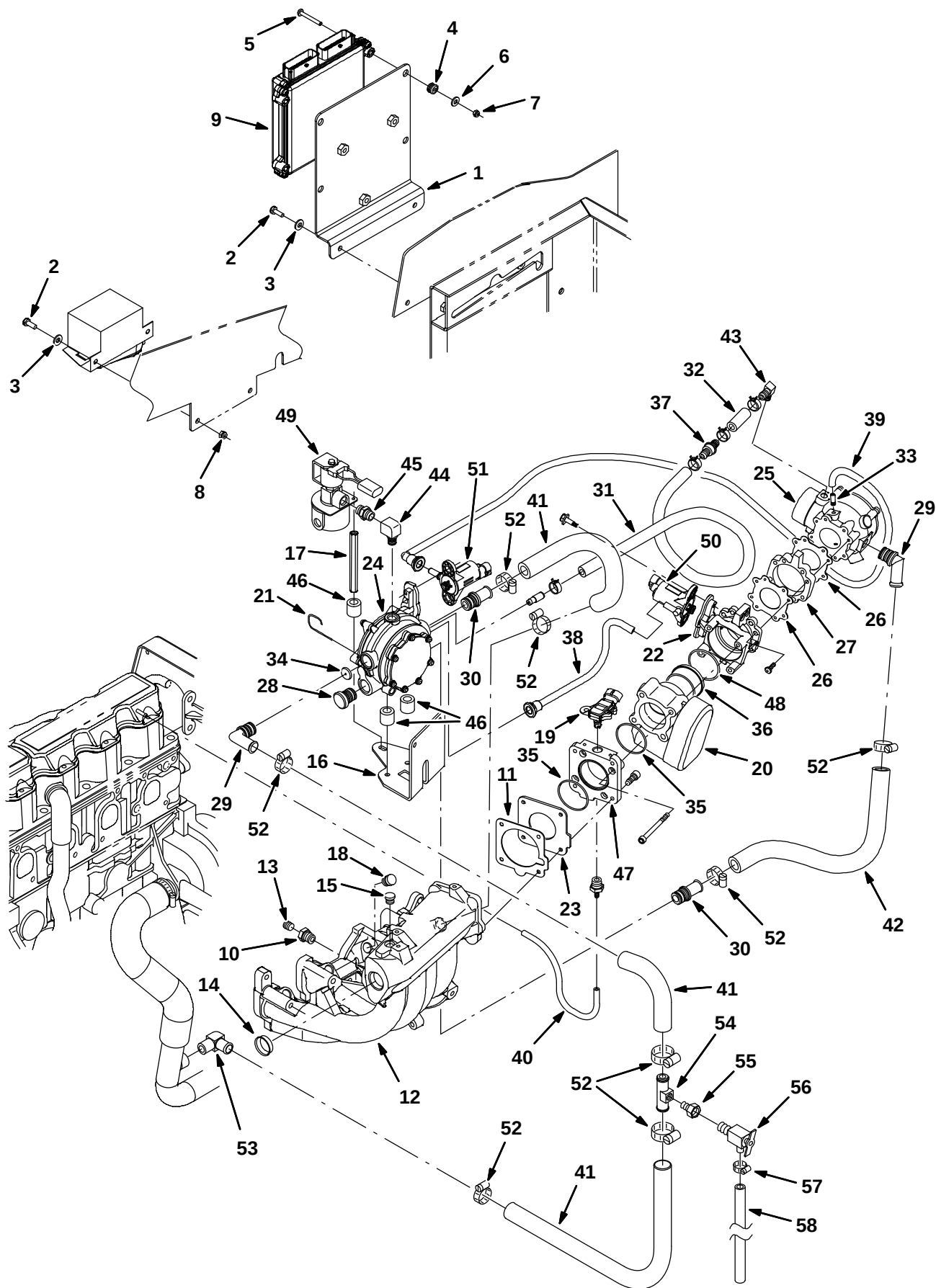
Fig. 15 – GM Engine EFI Group, LPG (0000-0046)
