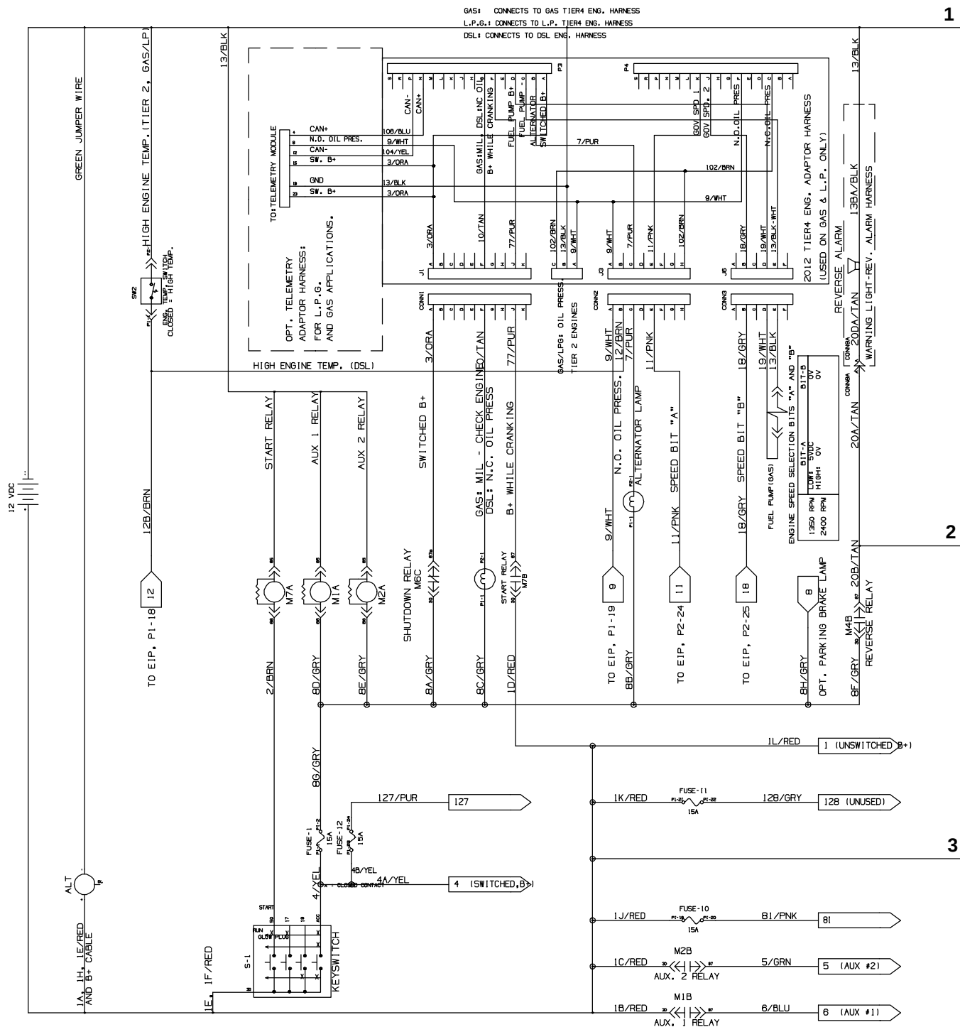
Fig. 93 – Mitsubishi Electrical Schematic (0500– )
