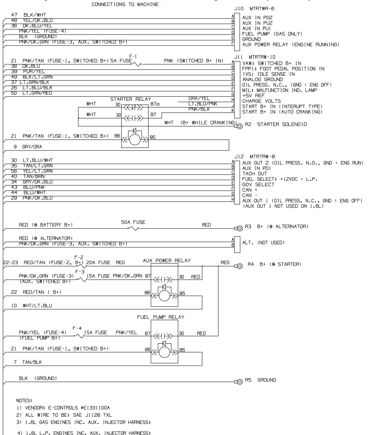
Fig. 88 – GM Electrical Schematic, Gas/LPG Engine Harness (0000–0046)
