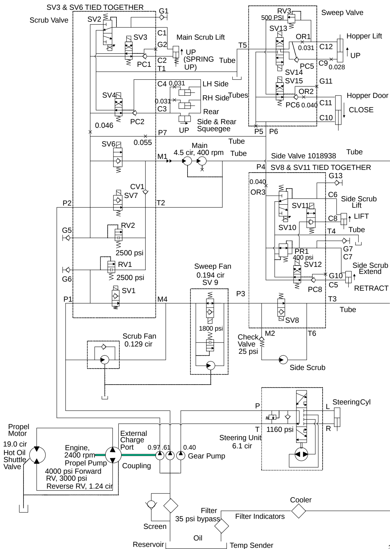
Fig. 72 – Hydraulic Schematic (0000 – 0131)
