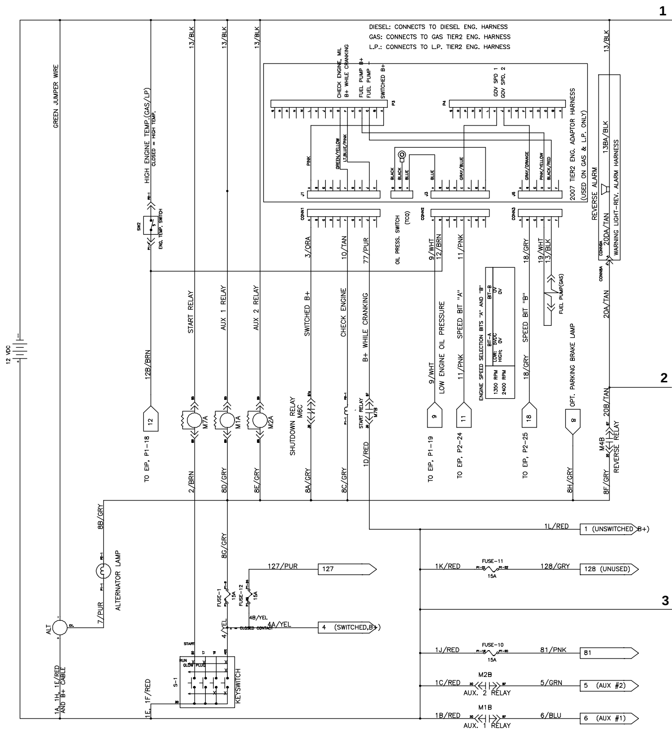
Fig. 87 – GM Electrical Schematic (xxxx-0499)
