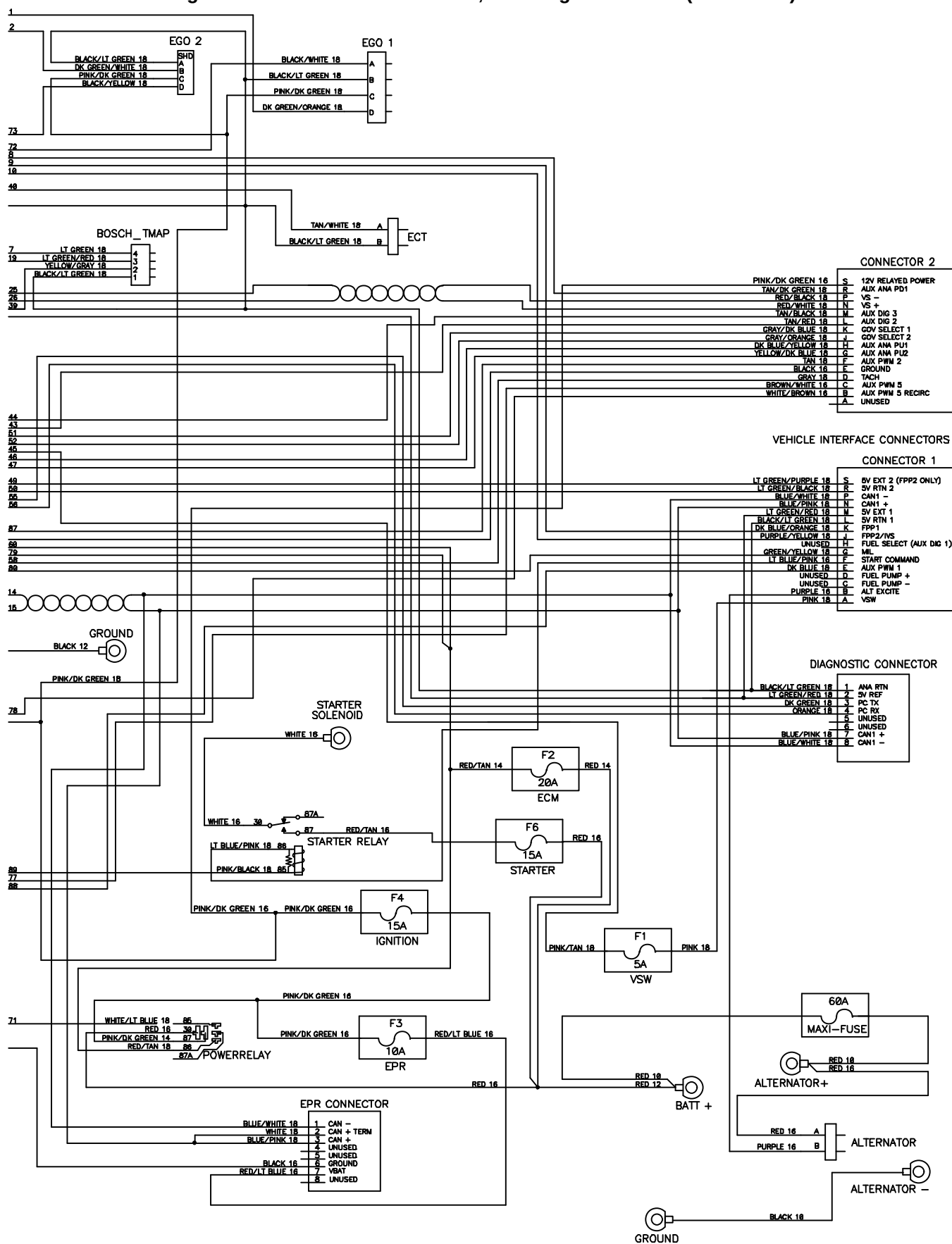
Fig. 92 – GM Electrical Schematic, LPG Engine Harness (0223–0499)
