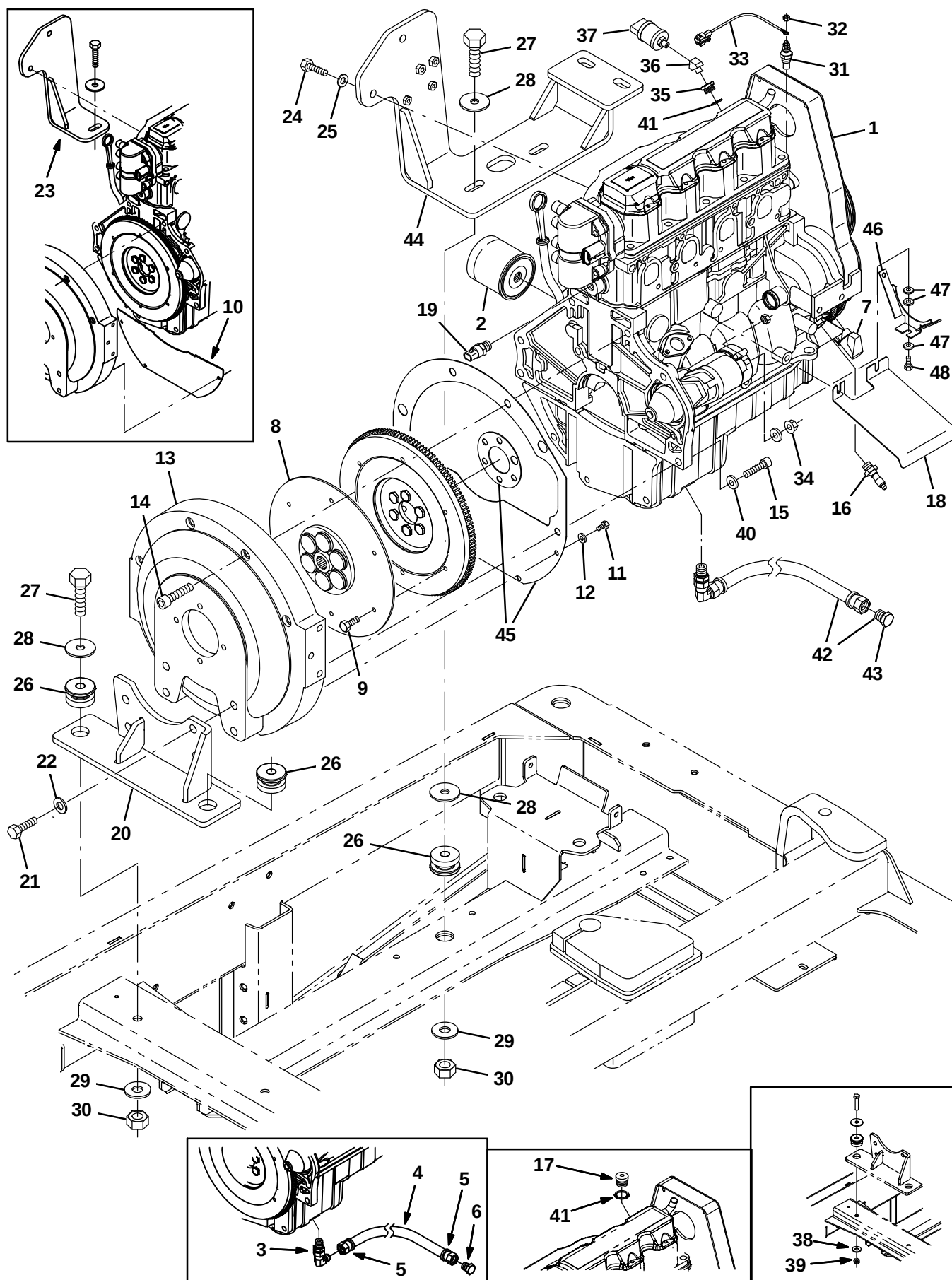
Fig. 11 – GM Engine and Mount Group (0000–0499)
