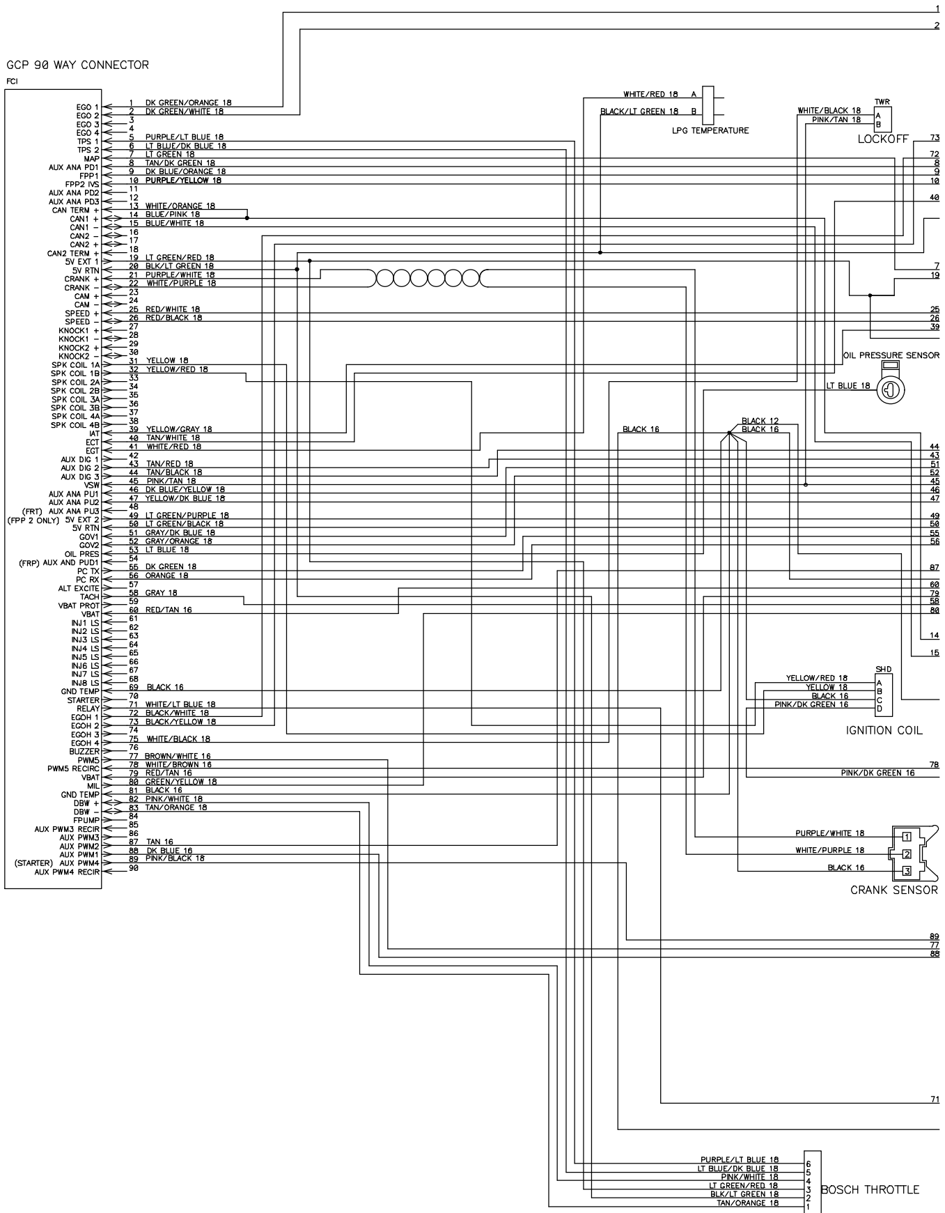
Fig. 91 – GM Electrical Schematic, LPG Engine Harness (0047-0222)
