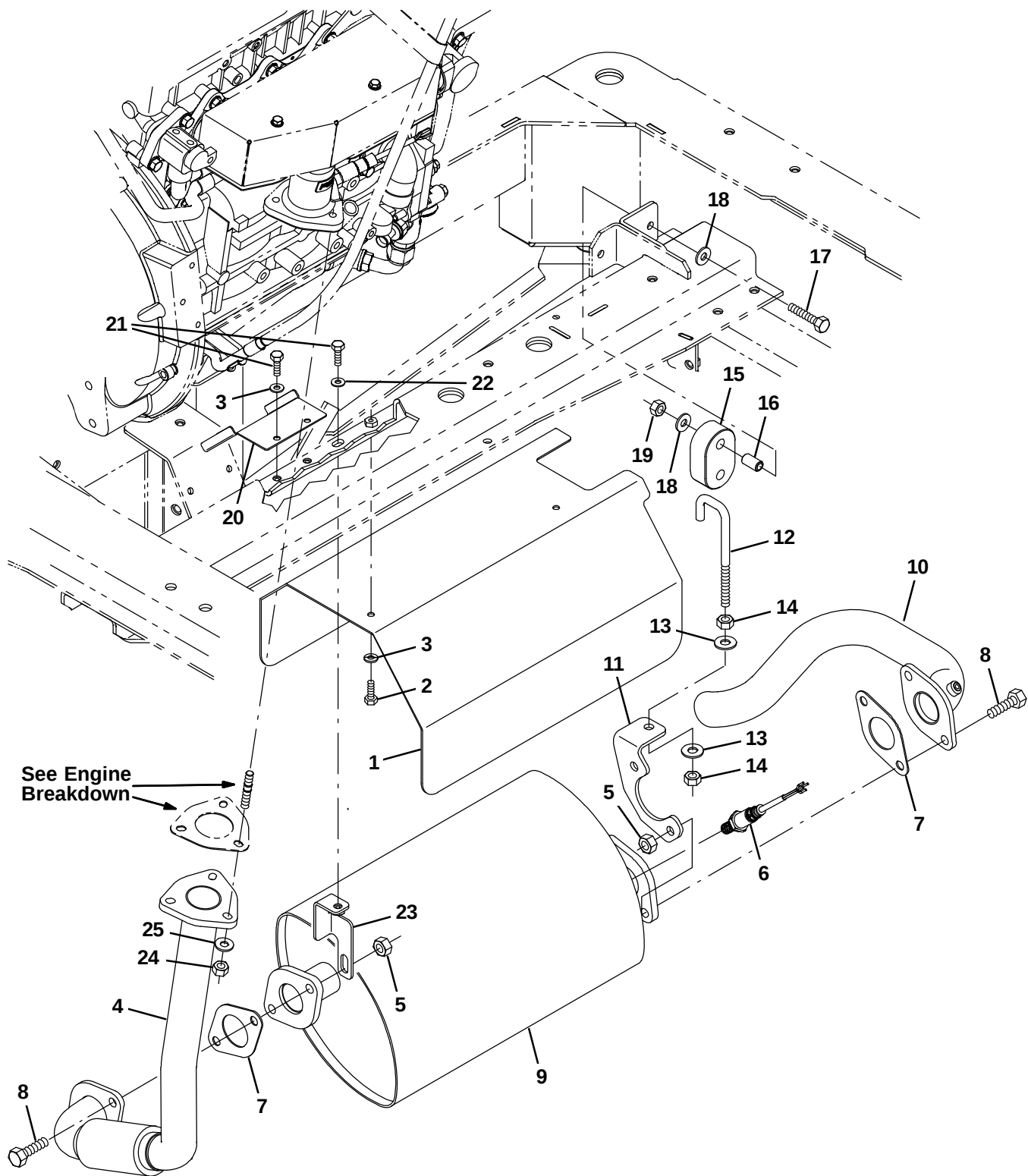
Fig. 37 – Mitsubishi Engine Muffler Group (0500– )
