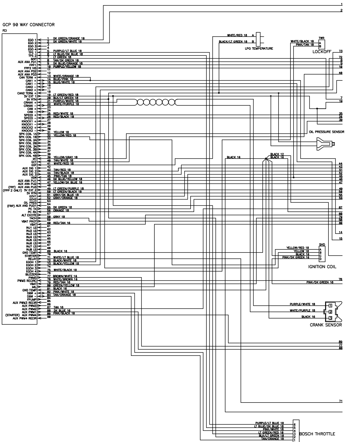
Fig. 92 – GM Electrical Schematic, LPG Engine Harness (0223-0499)
