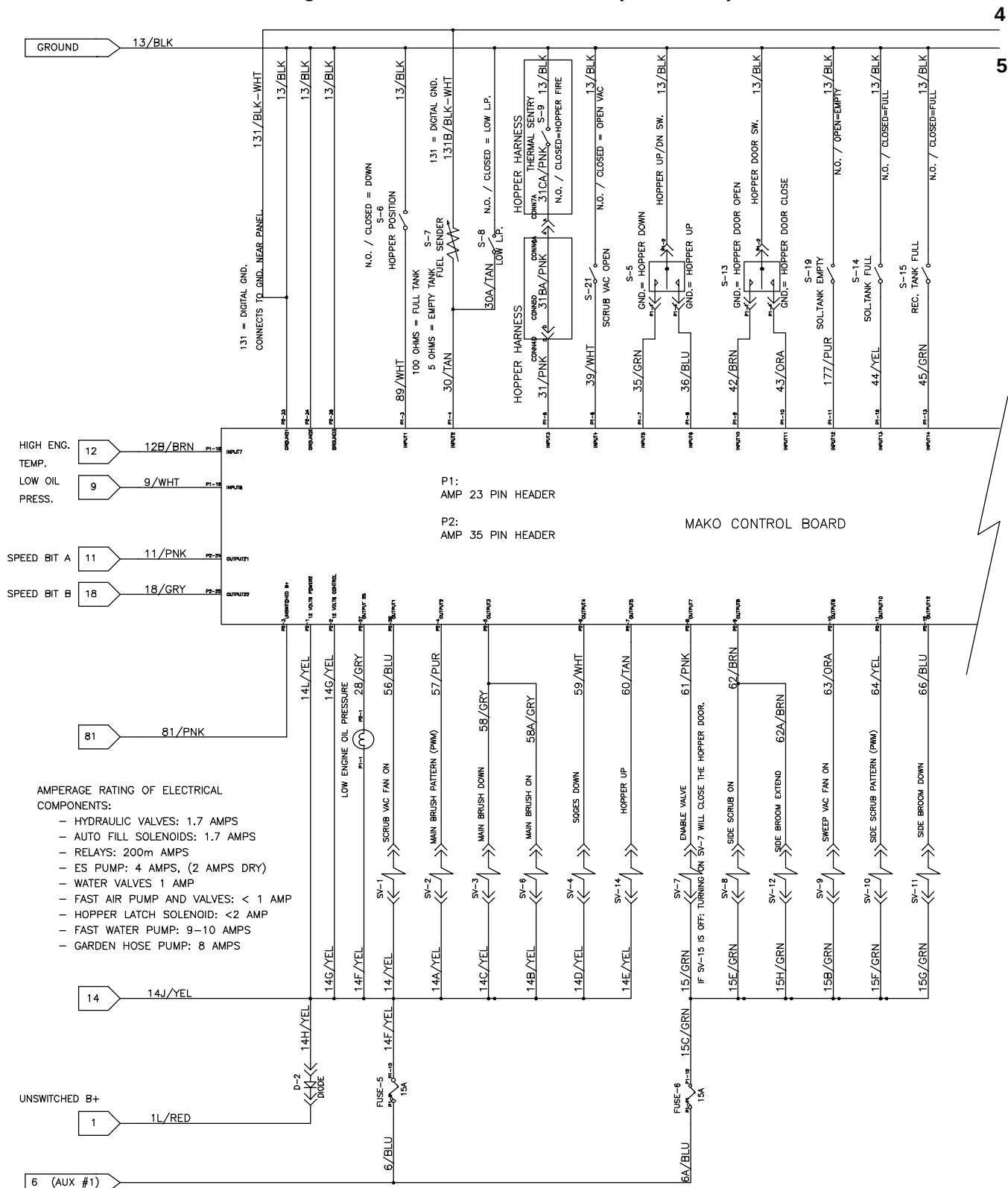
Fig. 86 – GM Electrical Schematic (0145-xxxx)
