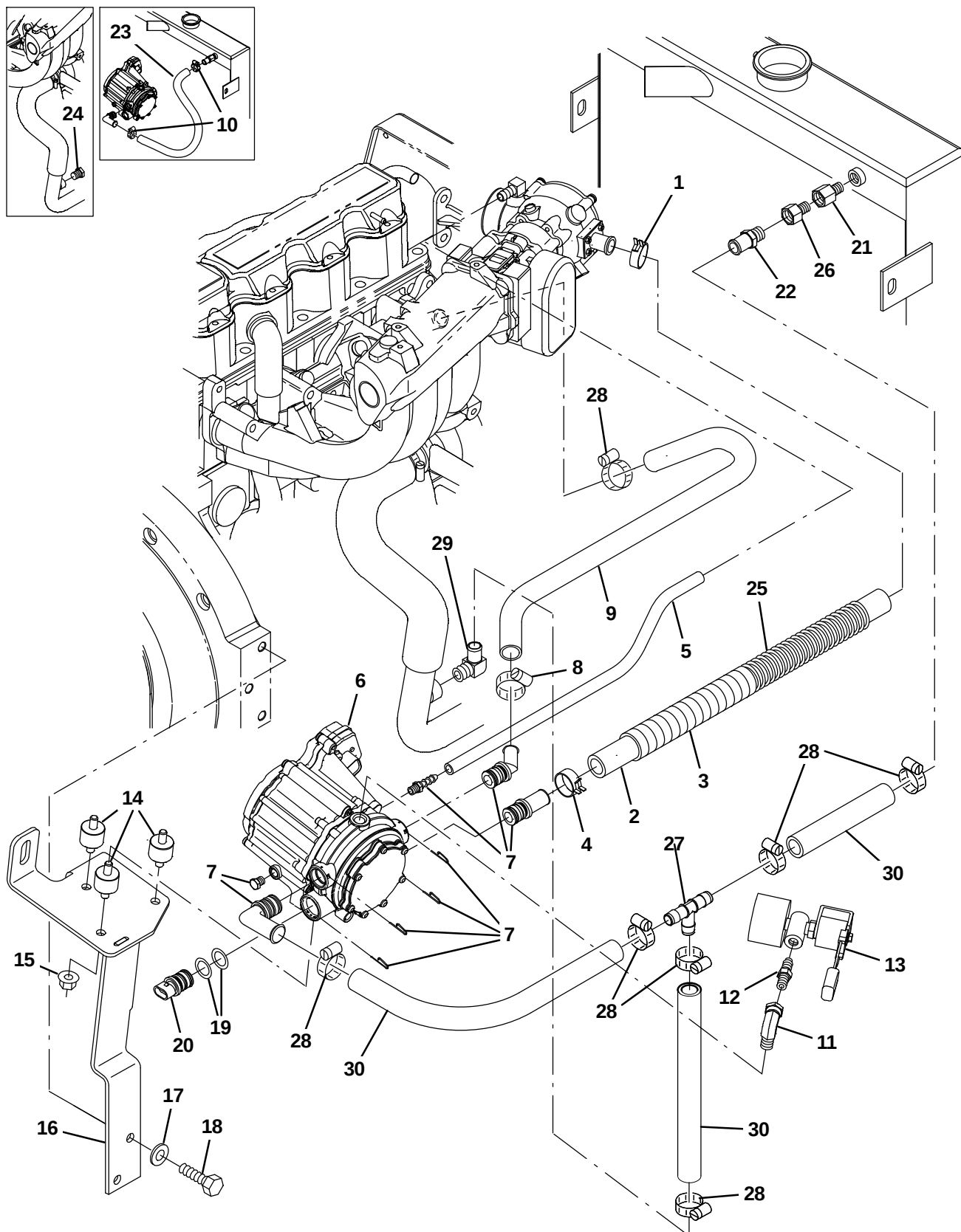
Fig. 18 – GM Engine Vaporizer Group, LPG (0223-0499)
