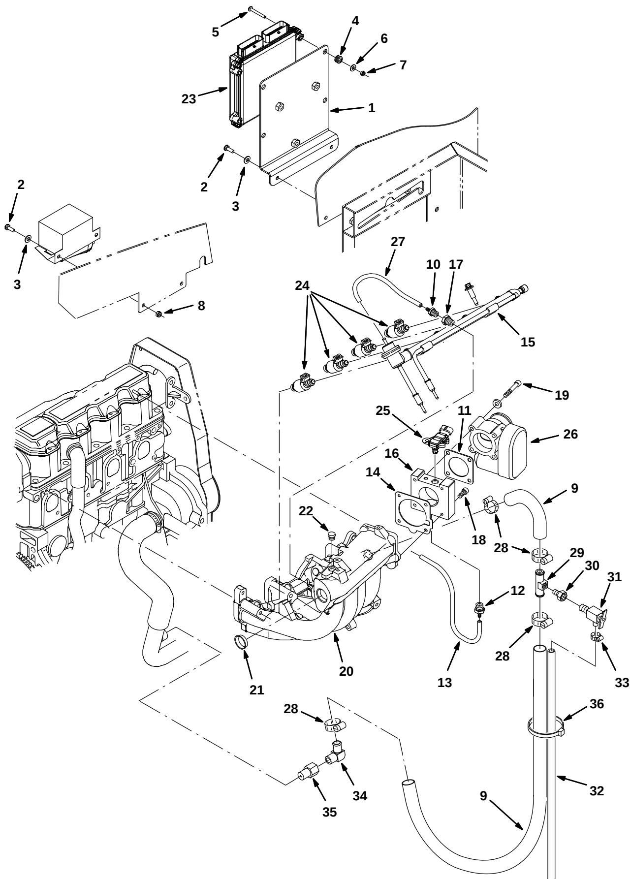
Fig. 12 – GM Engine EFI Group, Gasoline (0000-0046)
