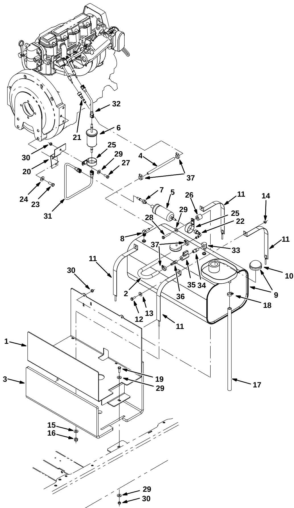
Fig. 19 – GM Engine Fuel Tank Group, Gasoline (0000-0046)
