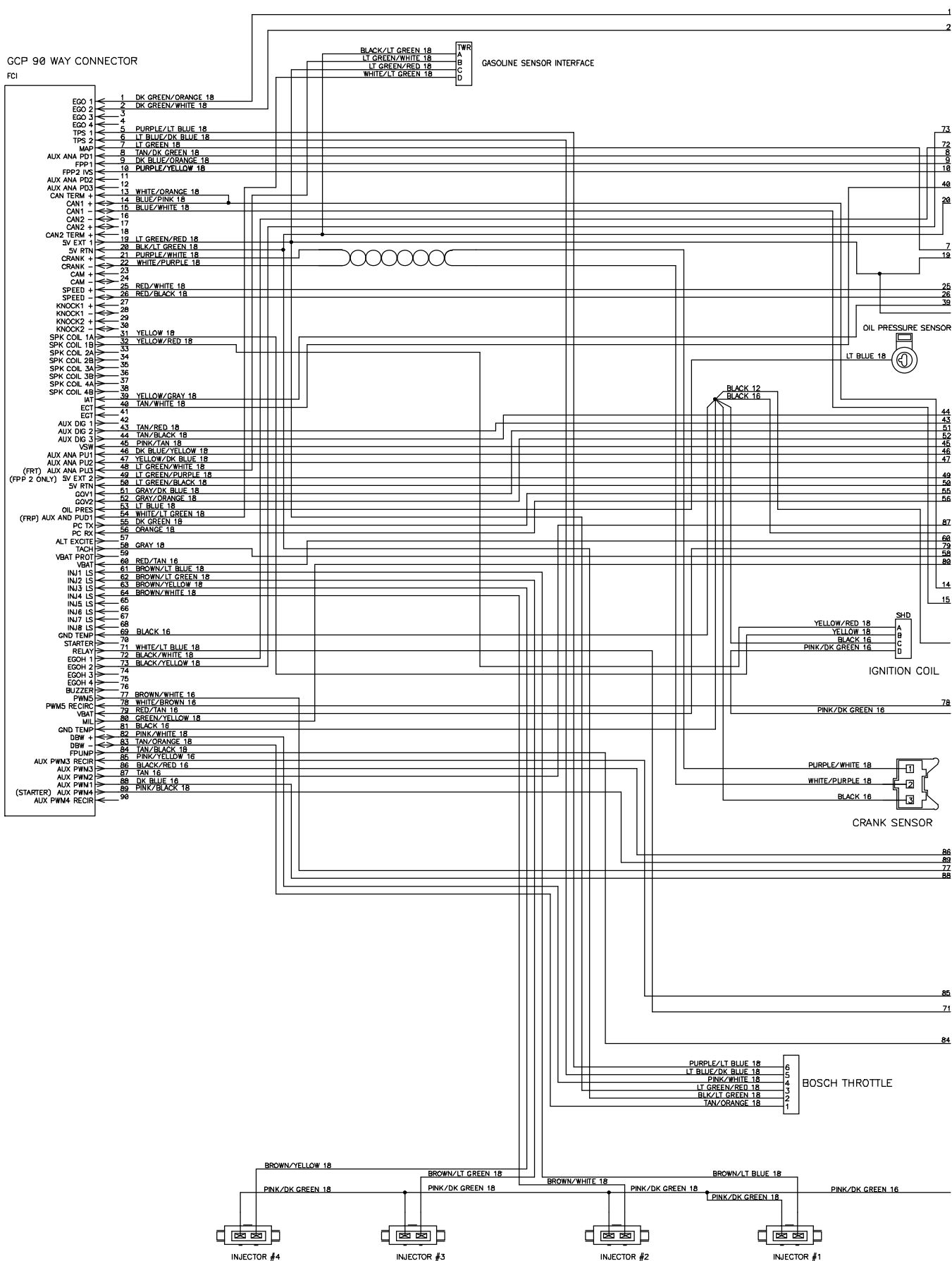
Fig. 89 – GM Electrical Schematic, Gas Engine Harness (0047-0222)
