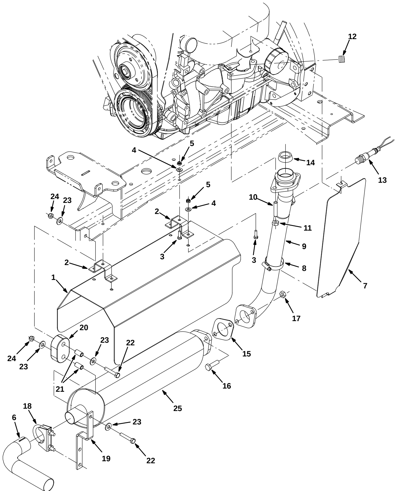
Fig. 25 – GM Engine Muffler Group (0000–0046)
