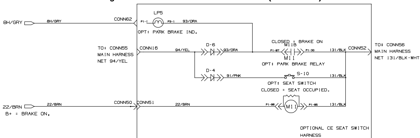
Fig. 93 – Mitsubishi Electrical Schematic (0500– )
