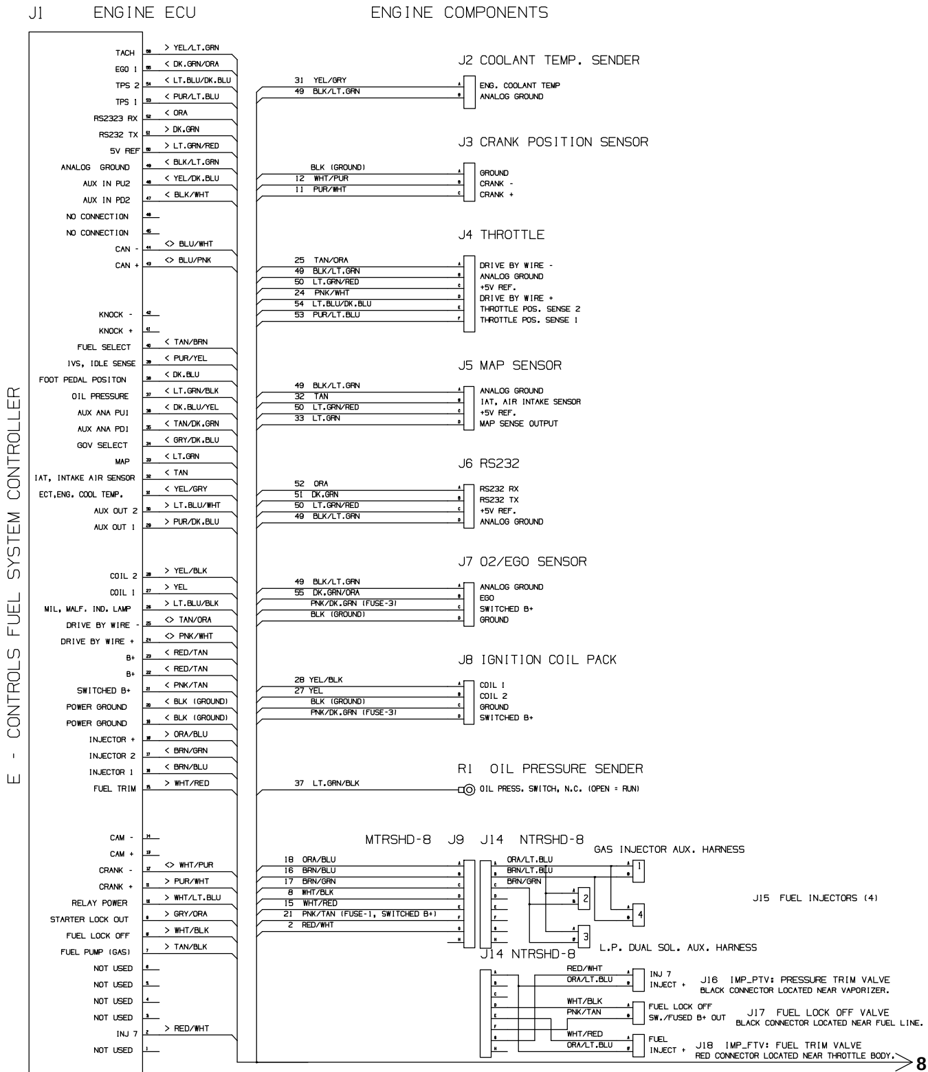
Fig. 88 – GM Electrical Schematic, Gas/LPG Engine Harness (0000-0046)
