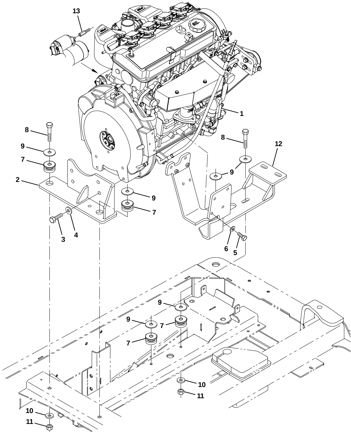
Fig. 30 – Mitsubishi Engine and Mount Group, Gas (0500– )
