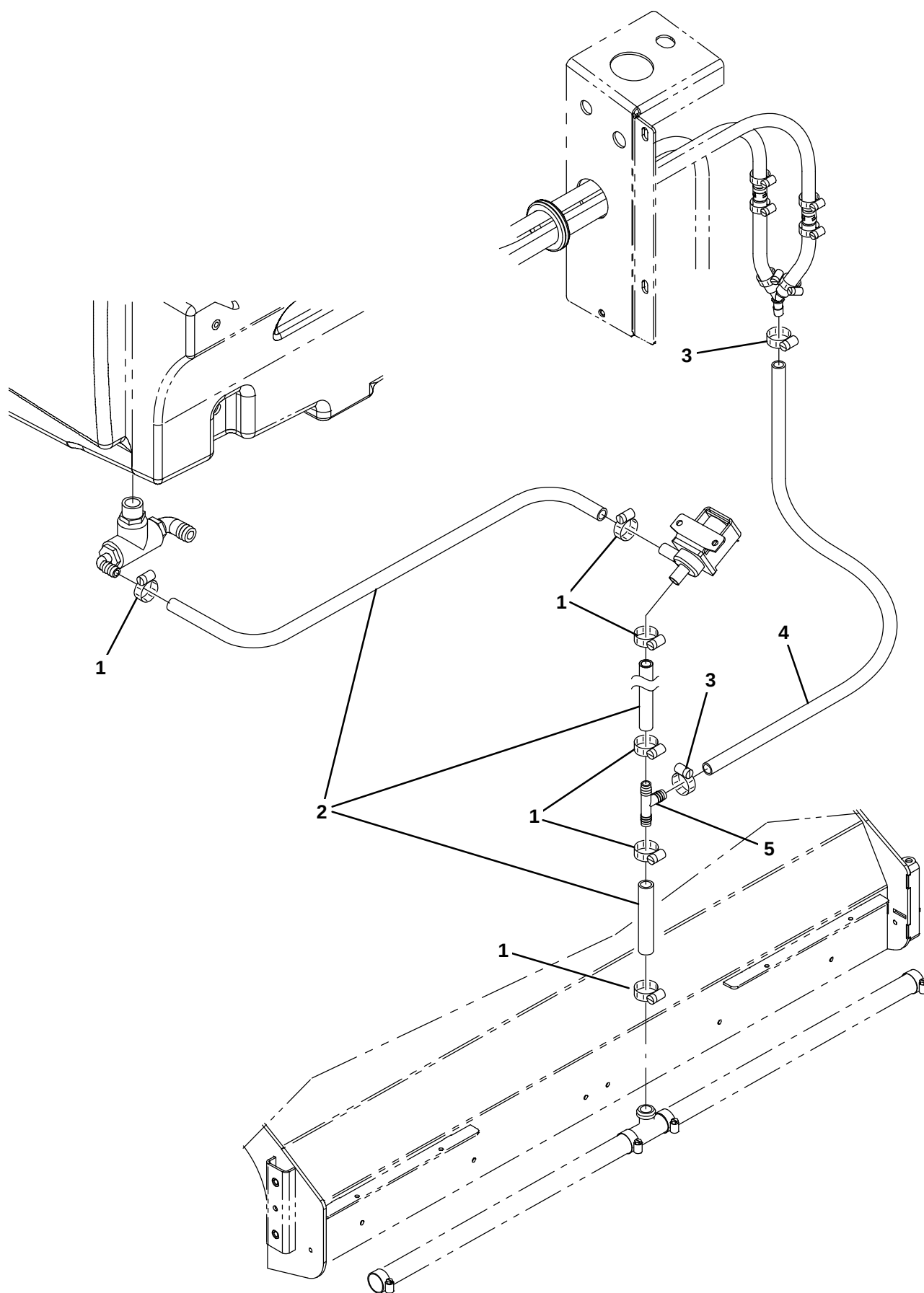
Fig. 15 – FaST Solution Supply Group (0146– )
