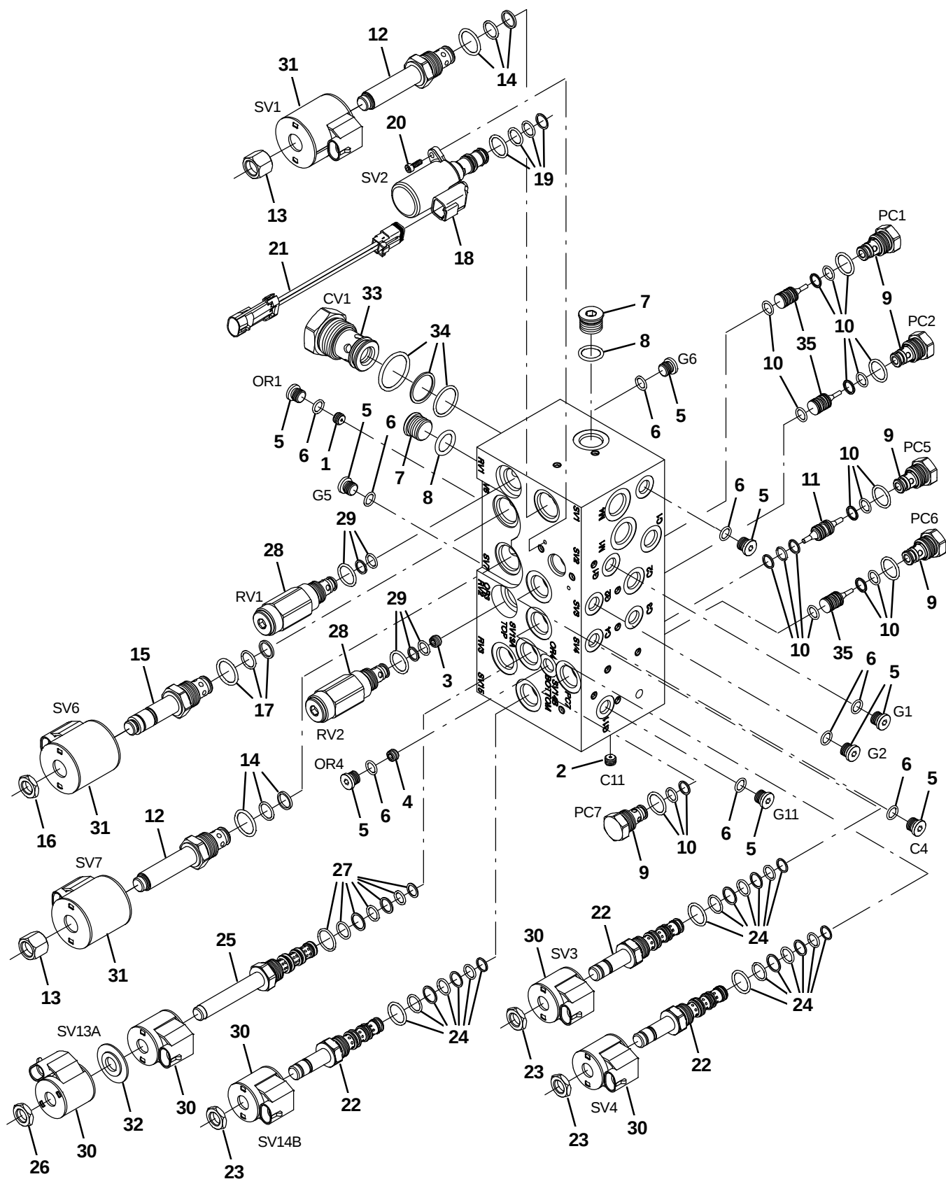
Fig. 13 – Hydraulic Valve Breakdown, 1072995
