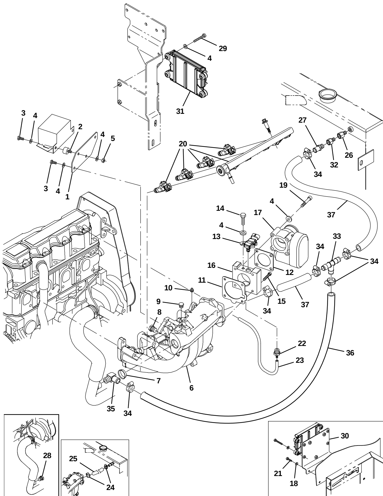
Fig. 14 – GM Engine EFI Group, Gasoline (0223-0499)
