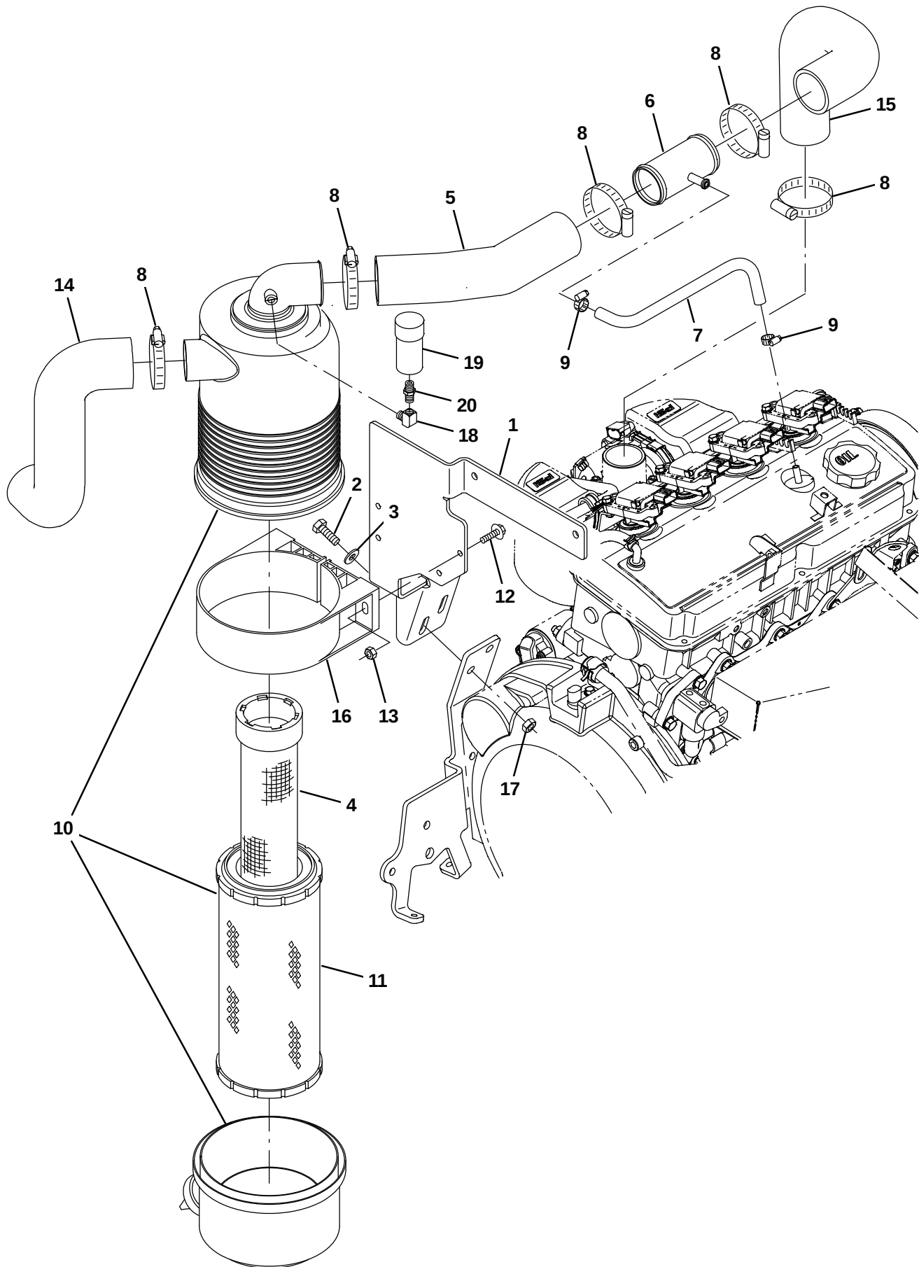
Fig. 34 – Mitsubishi Engine Air Cleaner Group, Gasoline (0500– )
