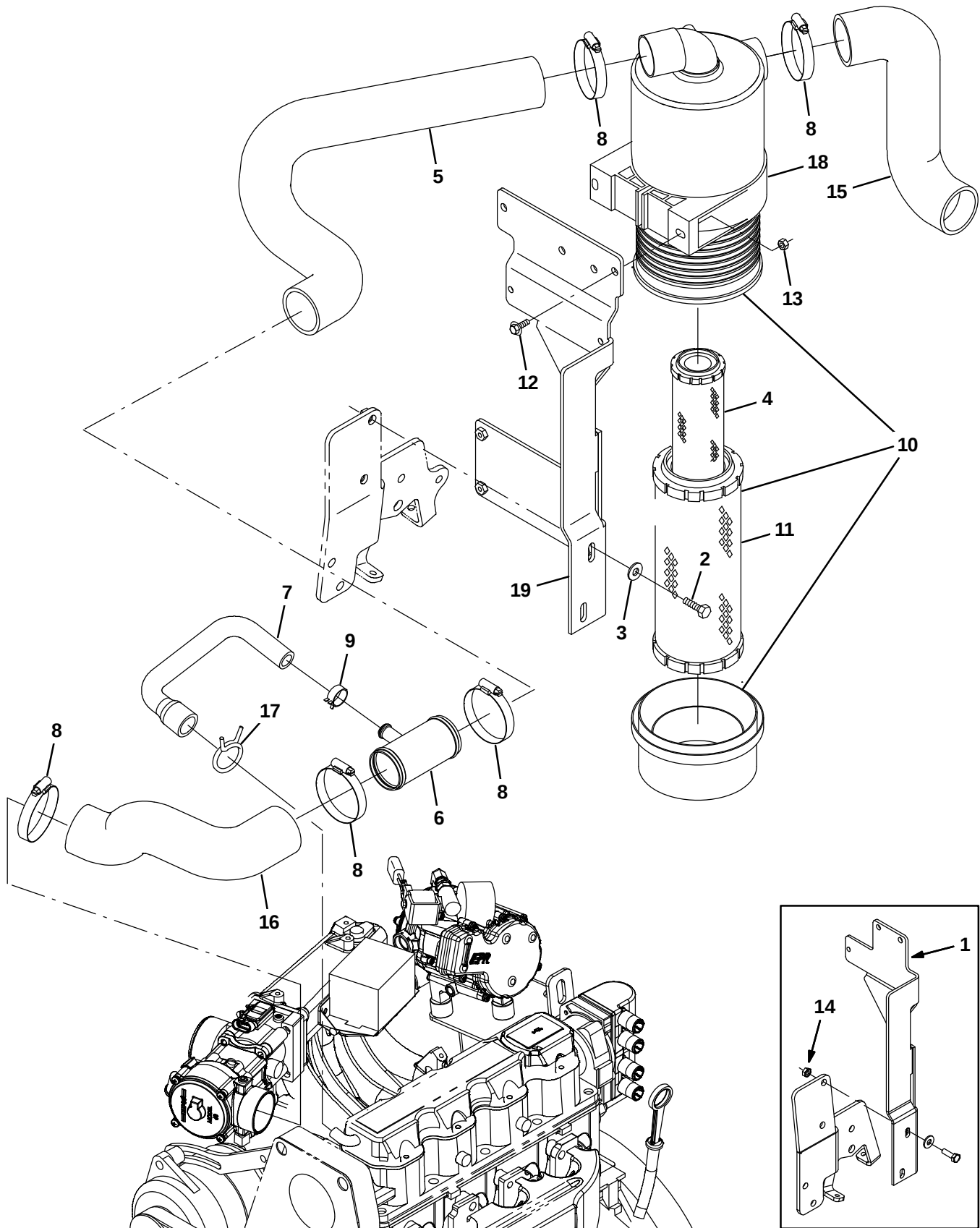
Fig. 23 – GM Engine Air Cleaner Group, LPG (0047–0499)
