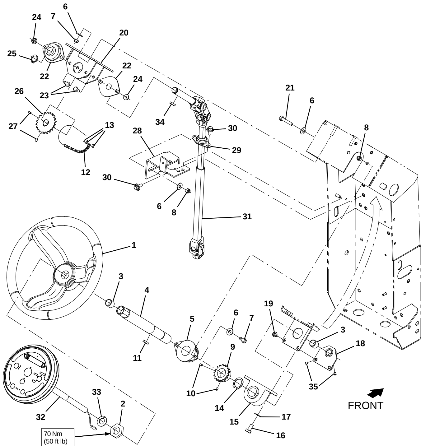
Fig. 5 – Steering Group
