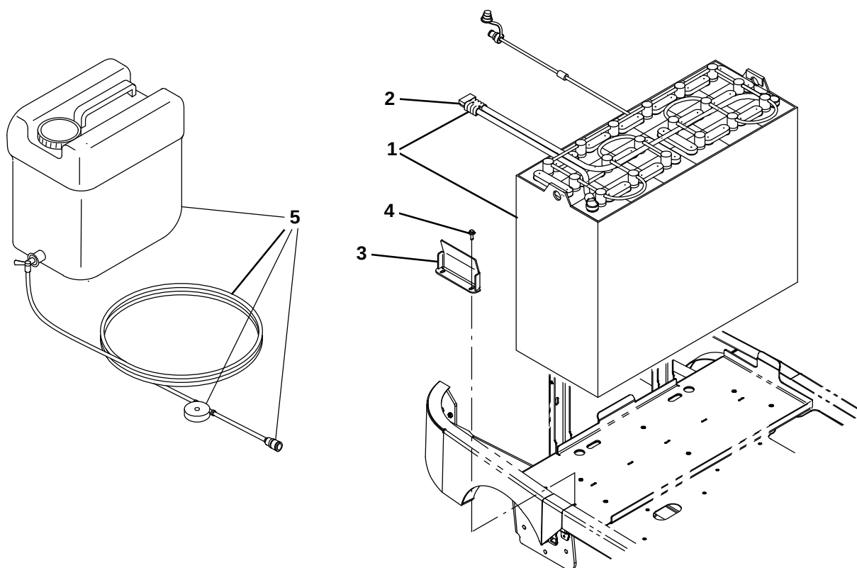
Fig. 37 – Battery Group
