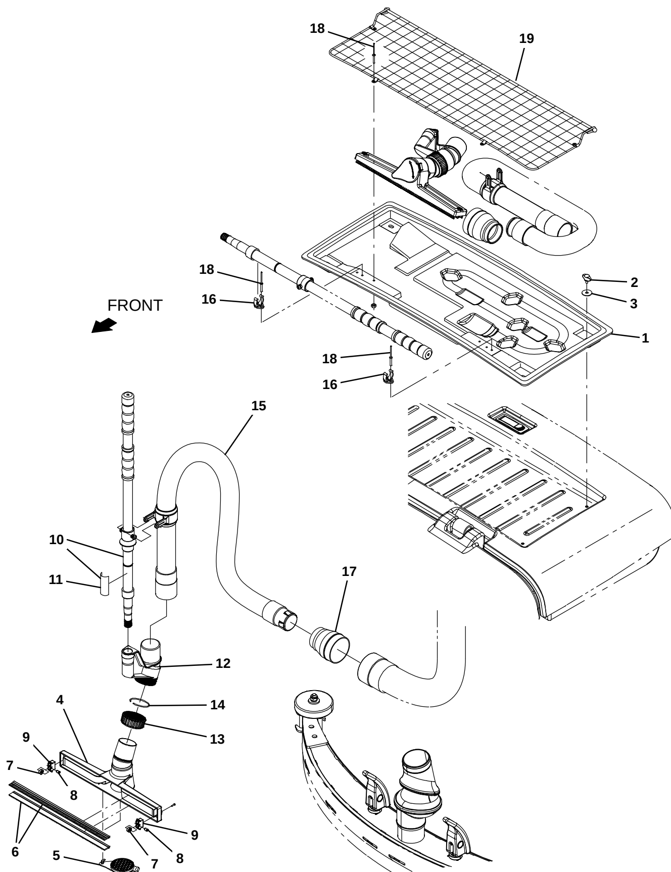
Fig. 34 – Vacuum Wand Kit
