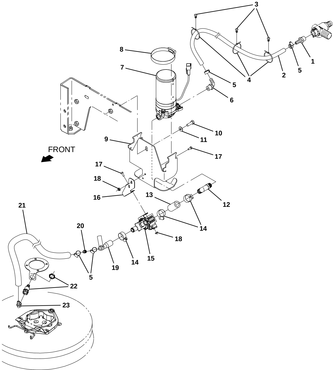
Fig. 10 – Scrubbing Side Brush Solution Supply Group
