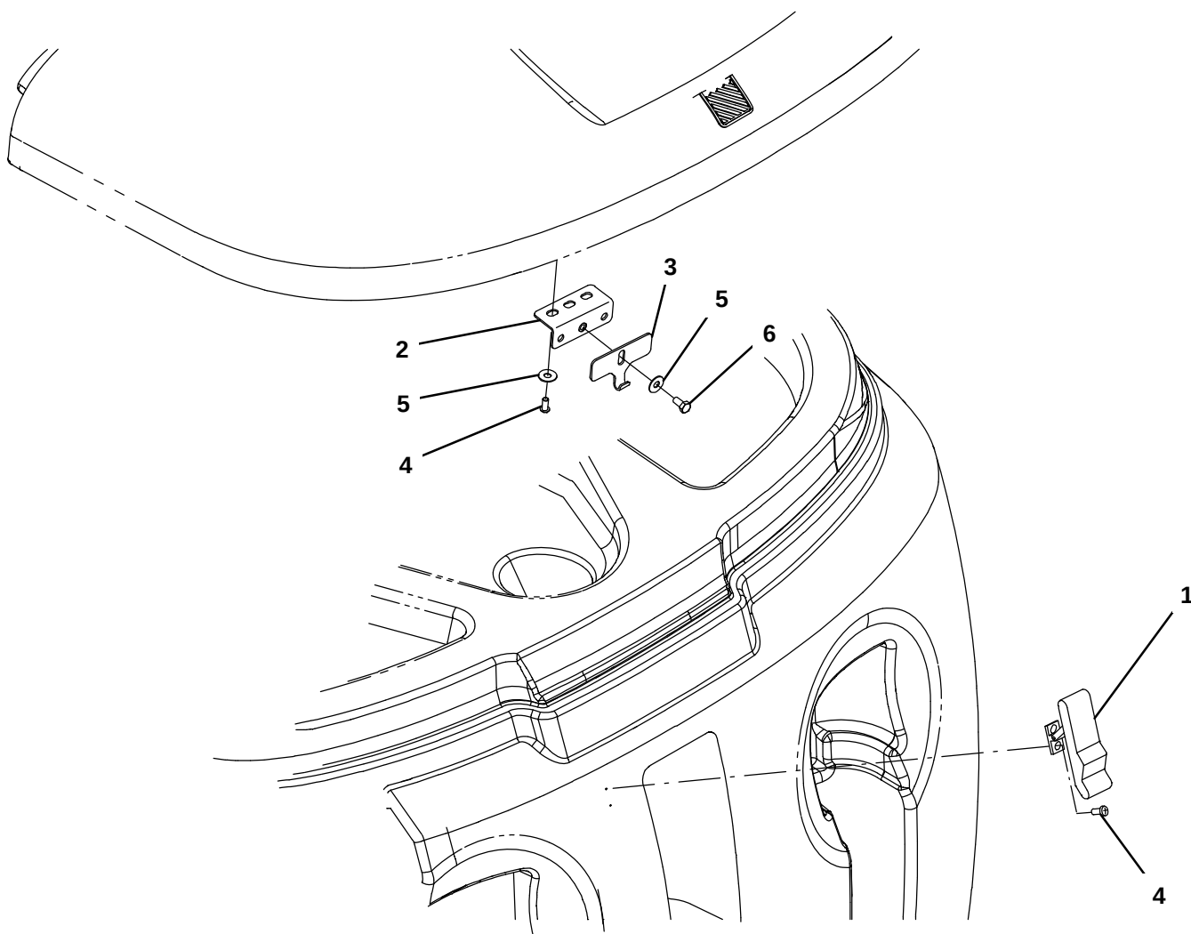
Fig. 40 – Transport Group
