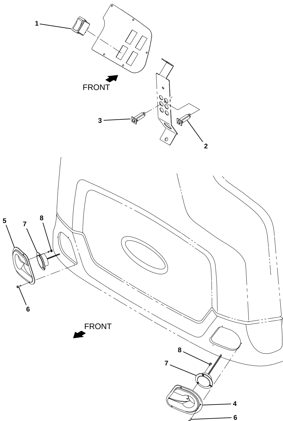
Fig. 1 – Headlight Group
