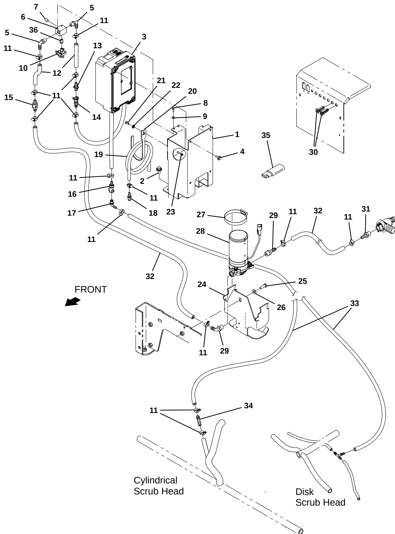
Fig. 30 – ec-H2O Solution Pump Group
