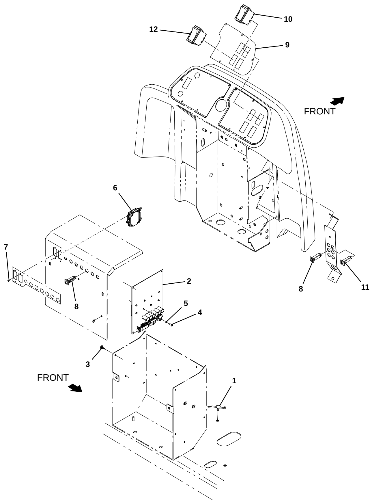
Fig. 24 – Pre-Sweep Electrical Group
