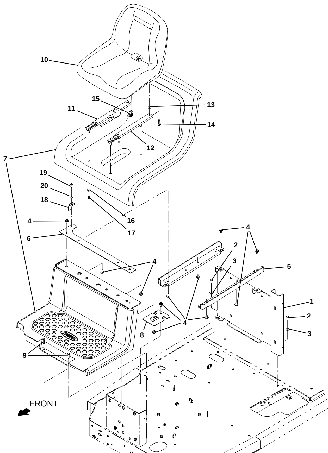
Fig. 8 – Seat Group
