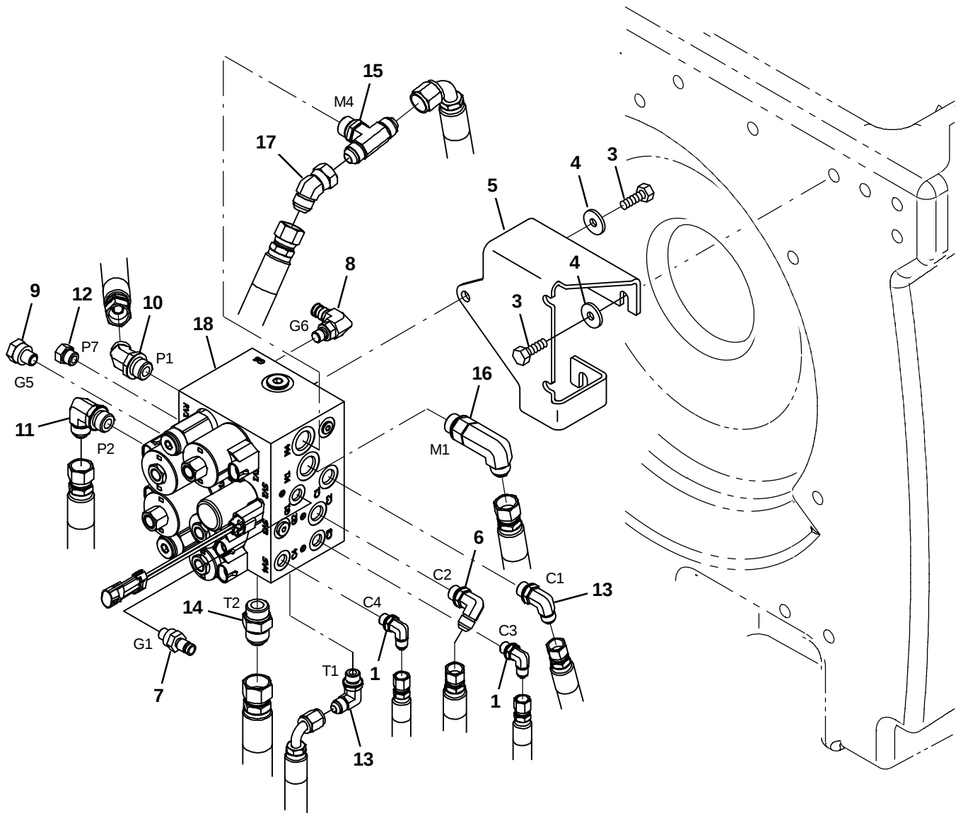
Fig. 60 – Hydraulic Valve Group
