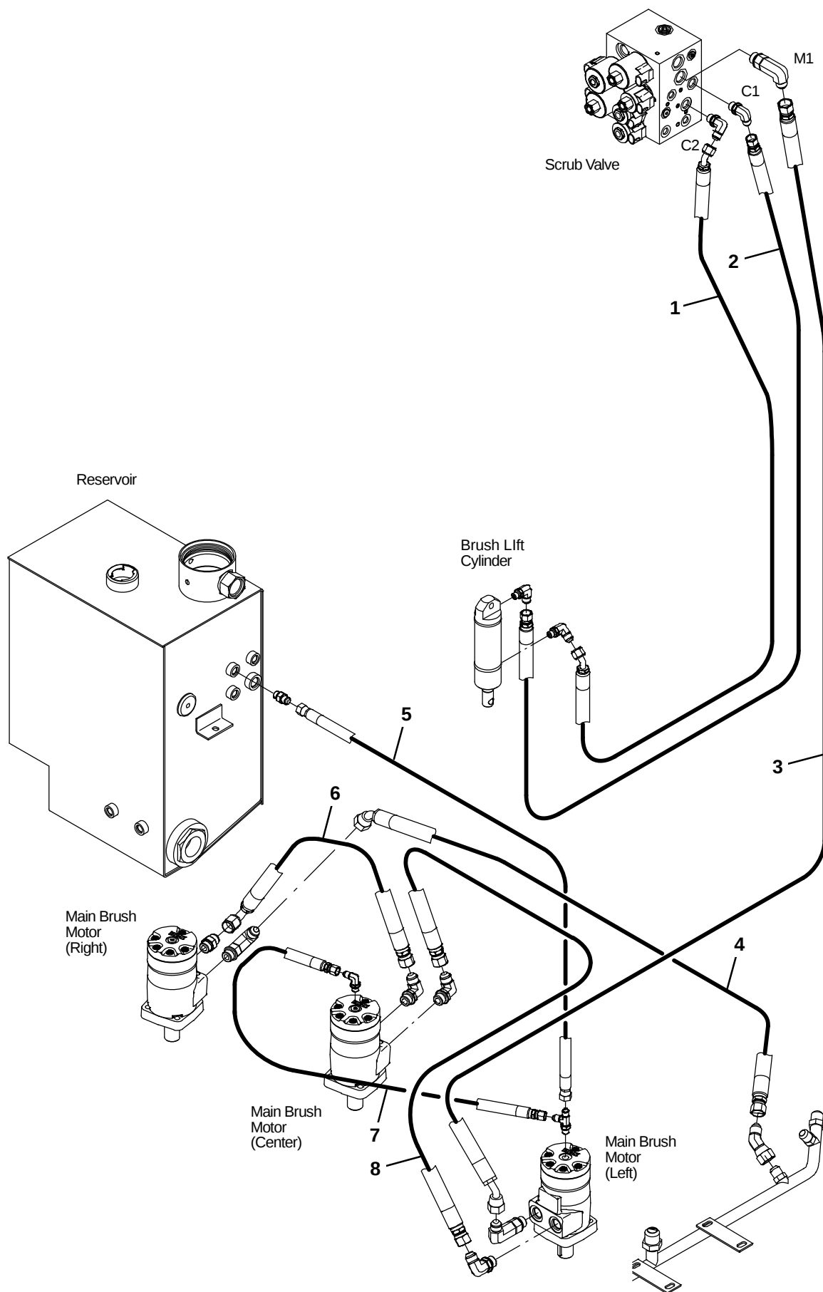
Fig. 55 – Hydraulic Hose Group, Disk Brush
