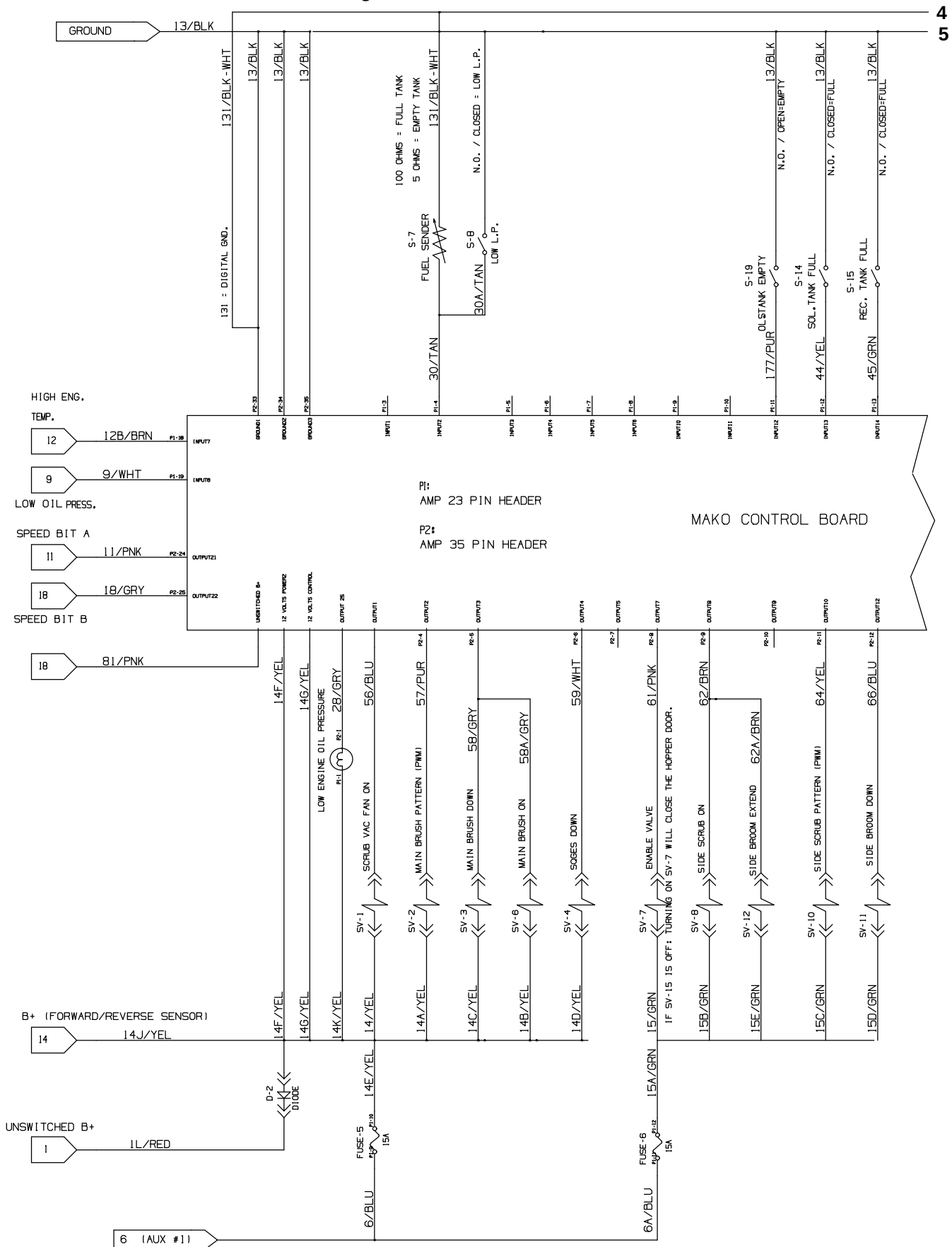
Fig. 61 – Electrical Schematic
