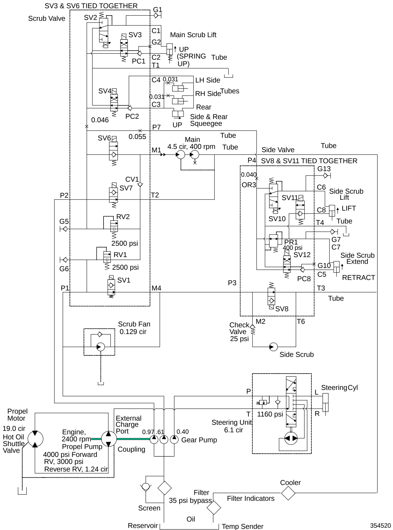
Fig. 49 – Hydraulic Schematic (0000–0042)
