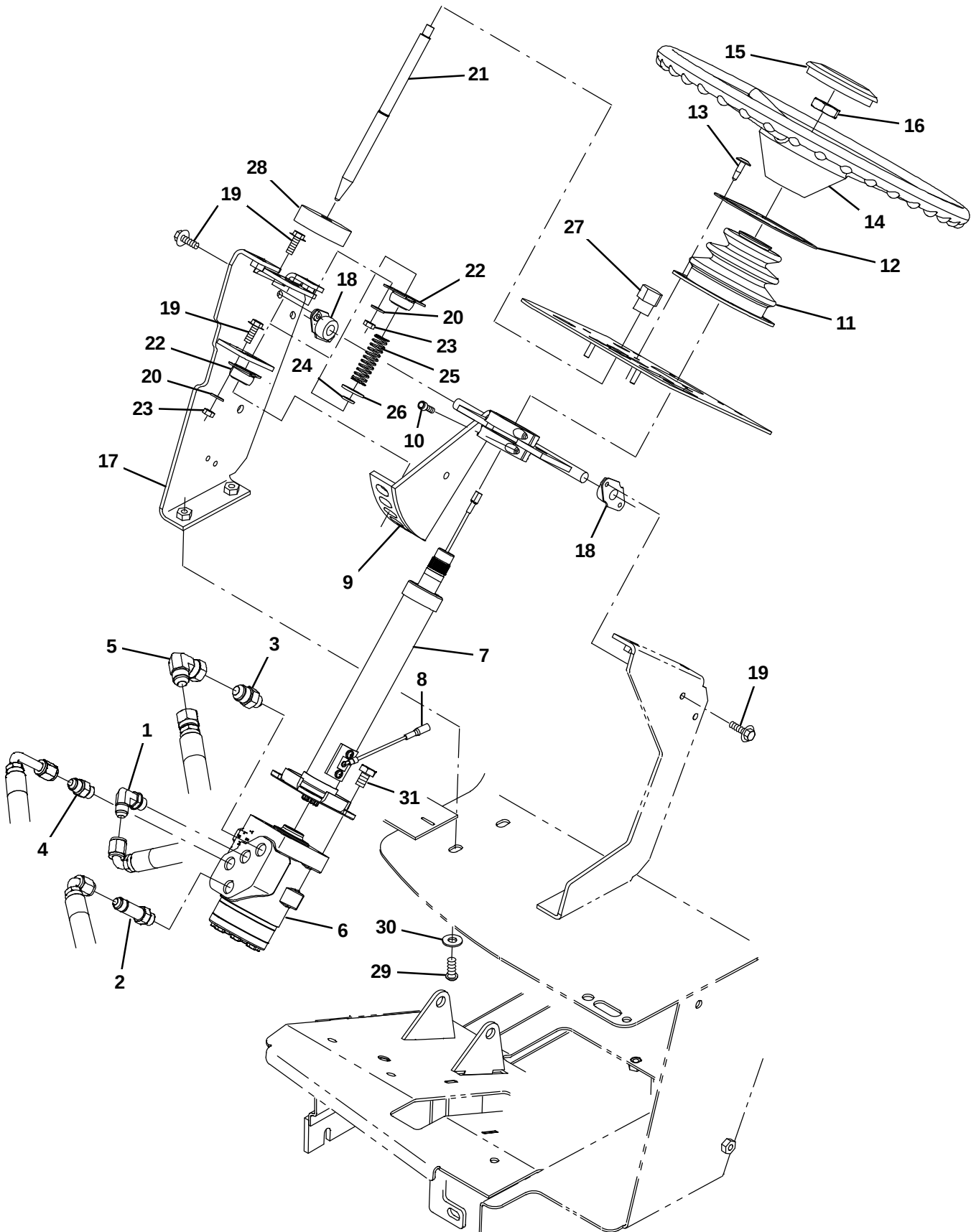
Fig. 8 – Steering Group
