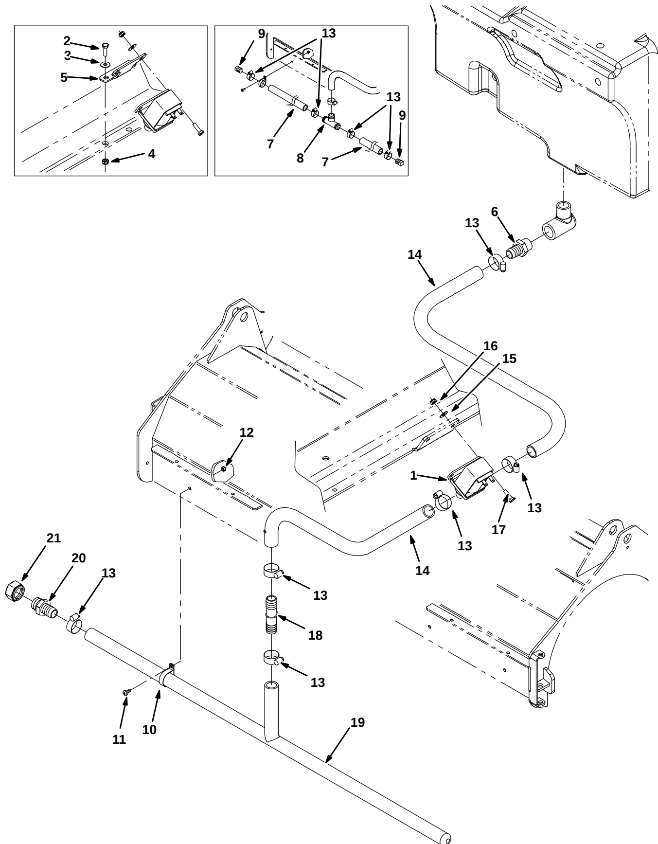
Fig. 44 – Solution Control Group, Cylindrical Scrub Head
