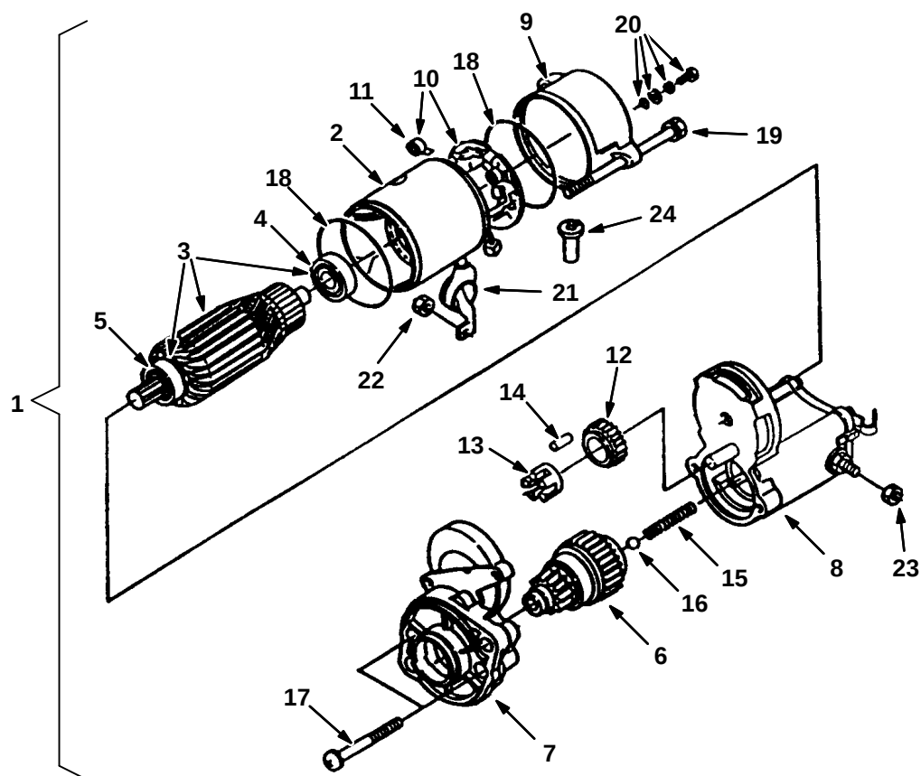
Fig. 14 – Starter Breakdown, 74405
