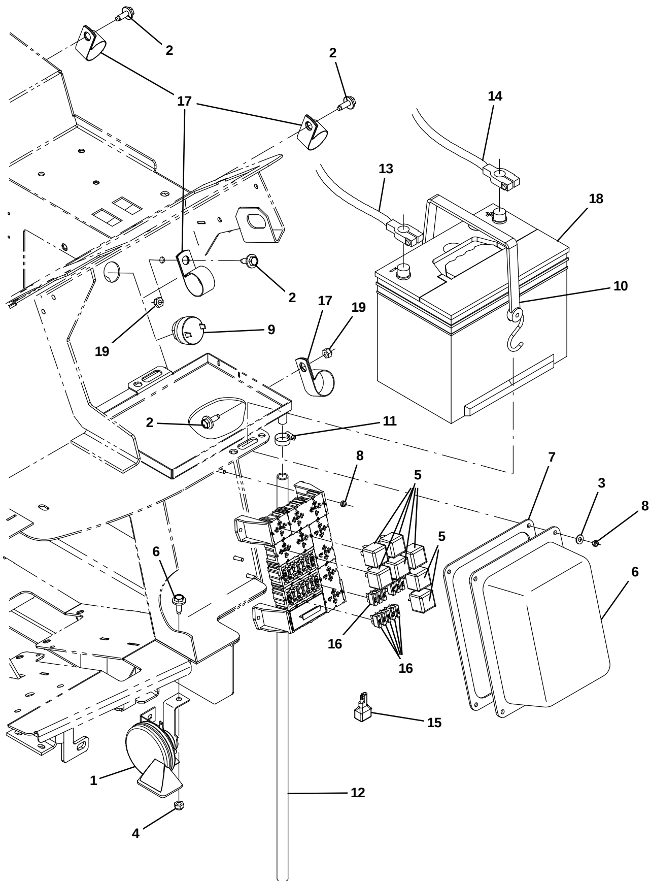
Fig. 22 – Battery and Electrical Group
