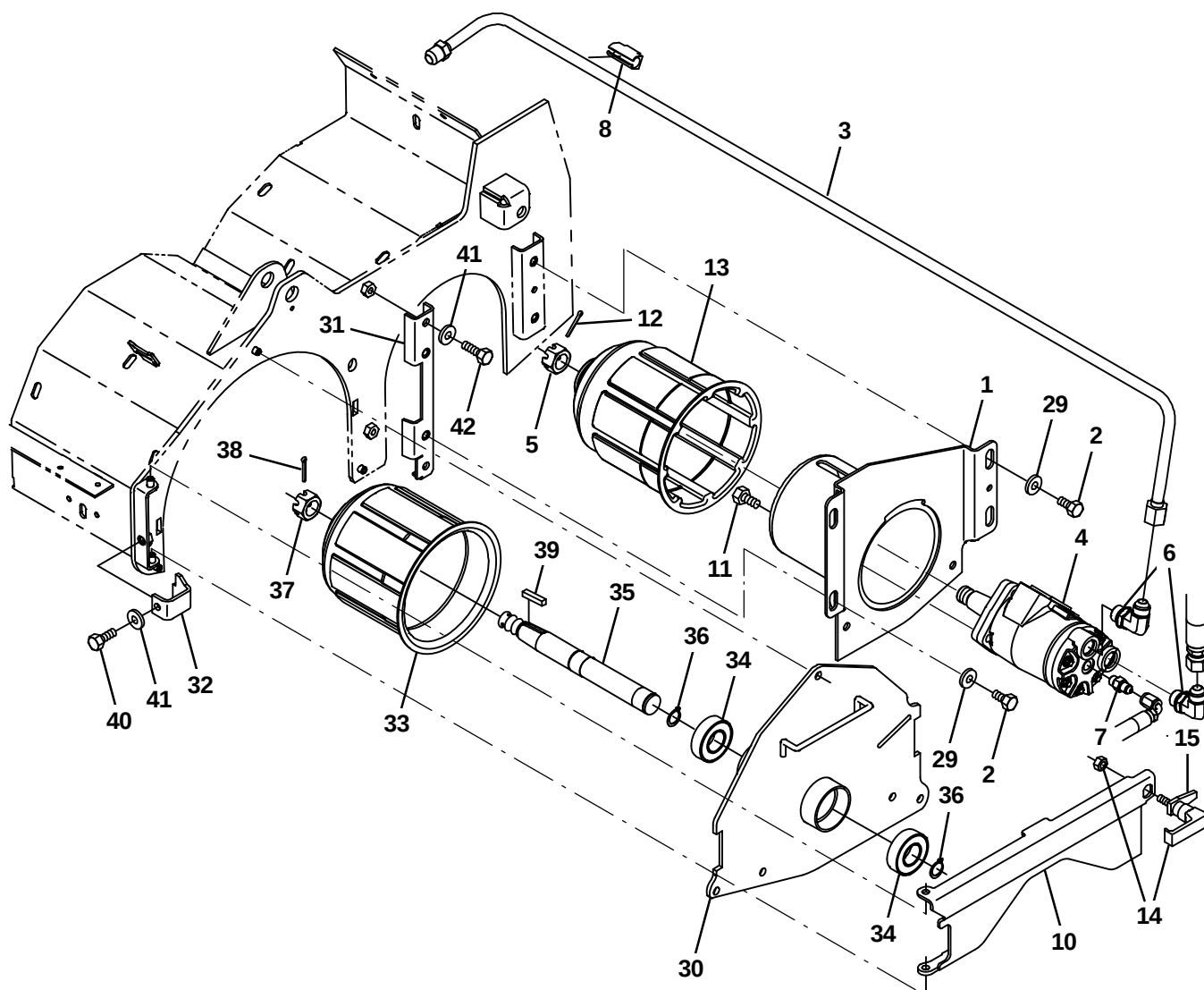
Fig. 27 – Cylindrical Scrub Brush Drive Group, Left Side
