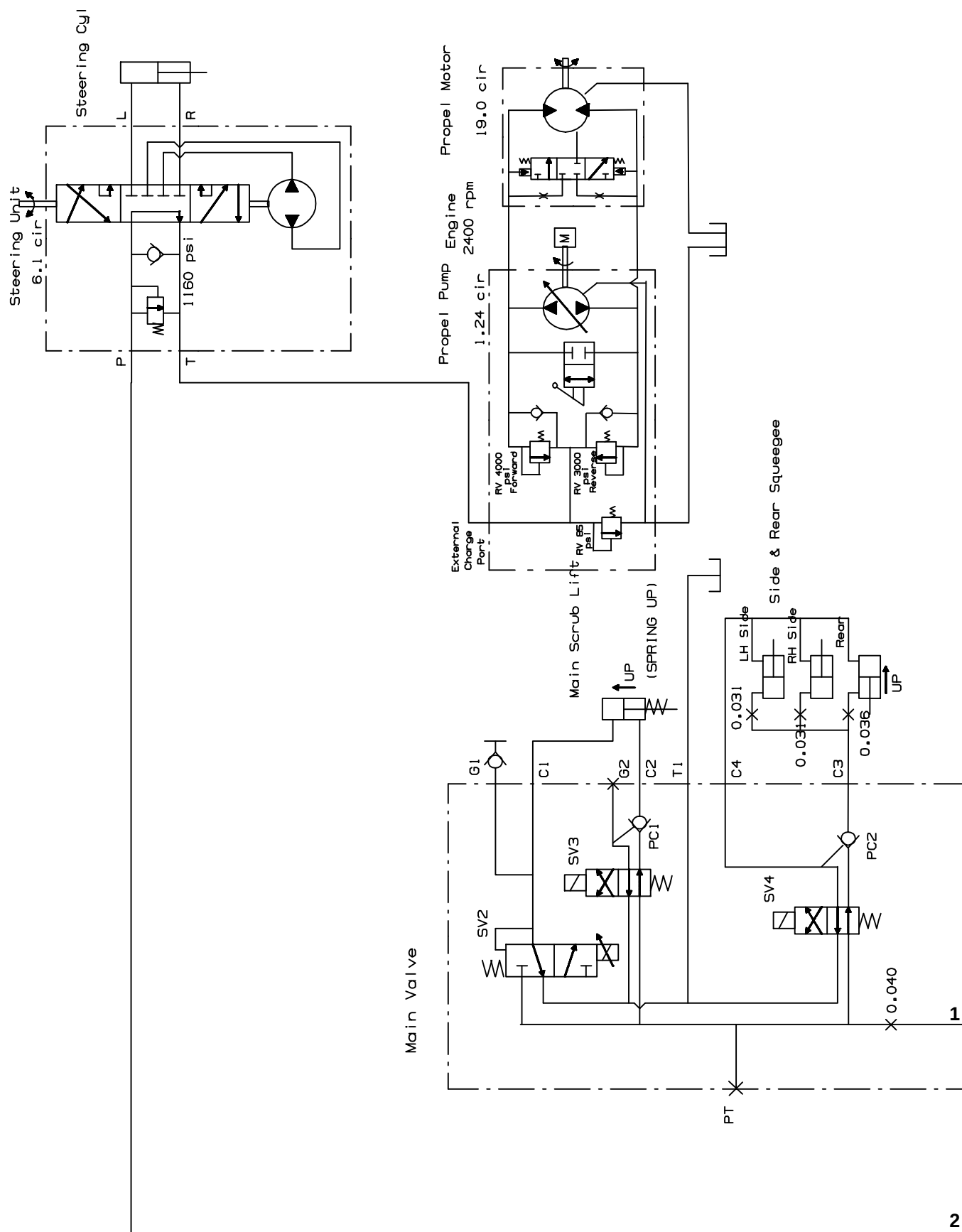
Fig. 50 – Hydraulic Schematic (0043–0244)
