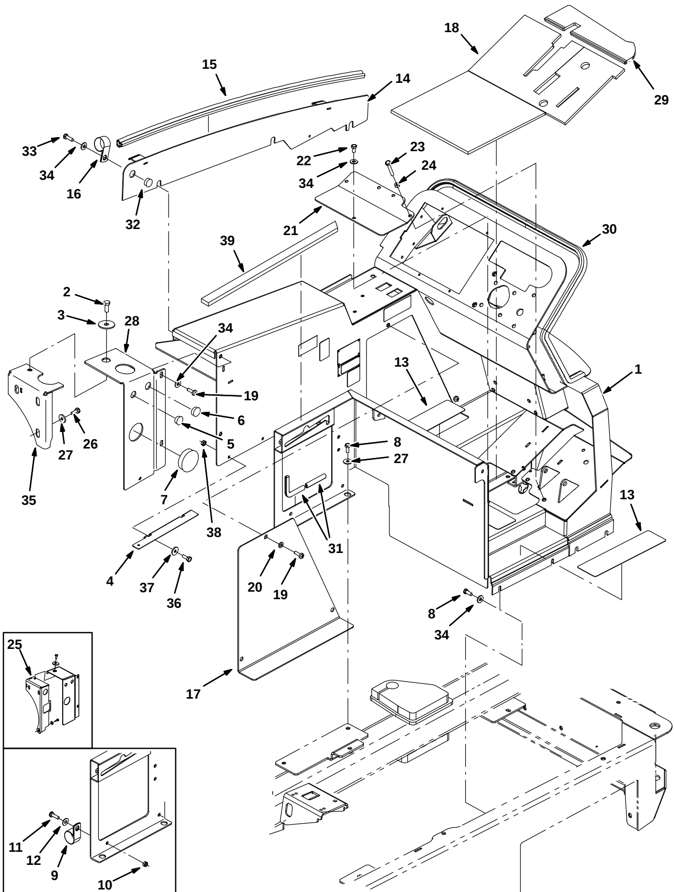
Fig. 4 – Operator Station
