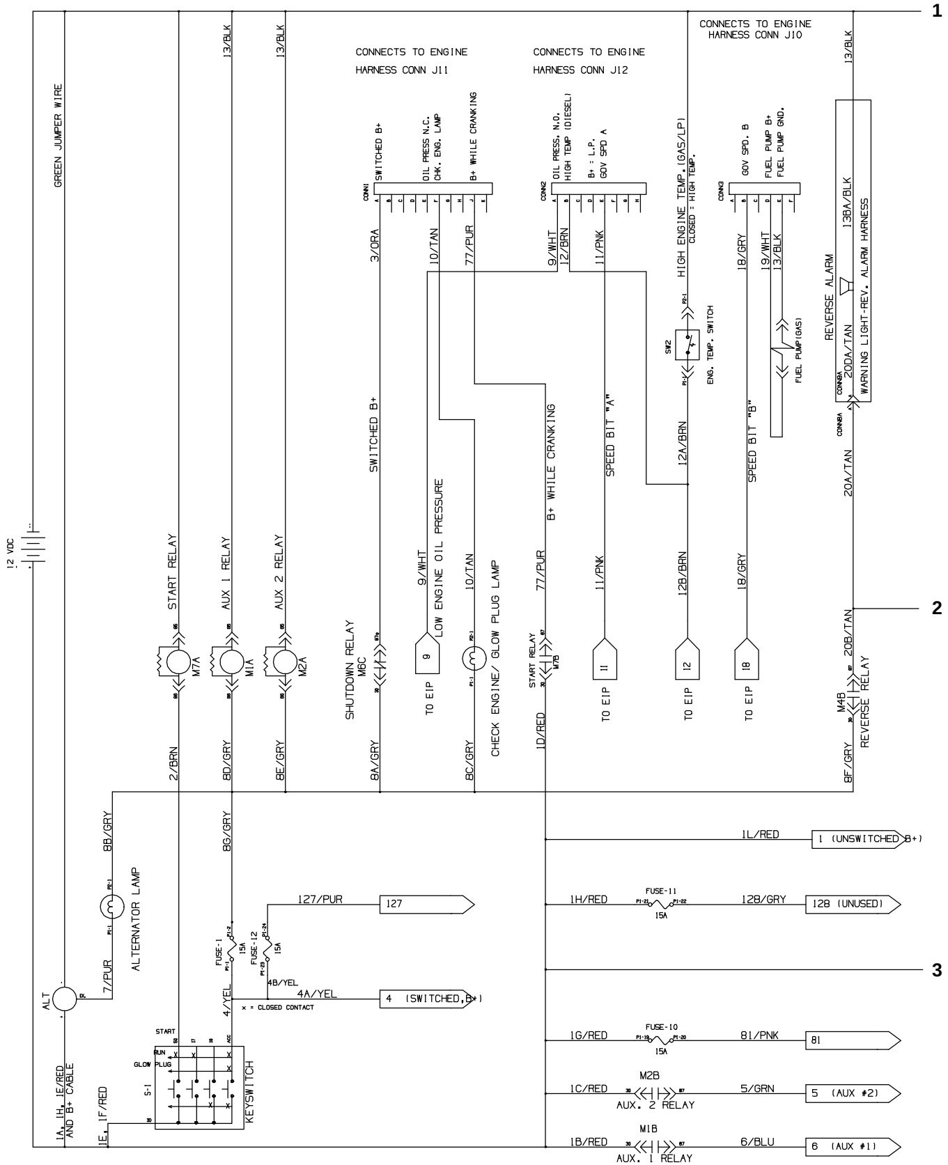
Fig. 61 – Electrical Schematic
