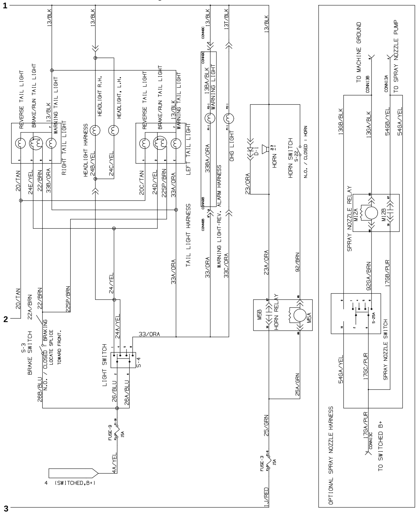
Fig. 61 – Electrical Schematic
