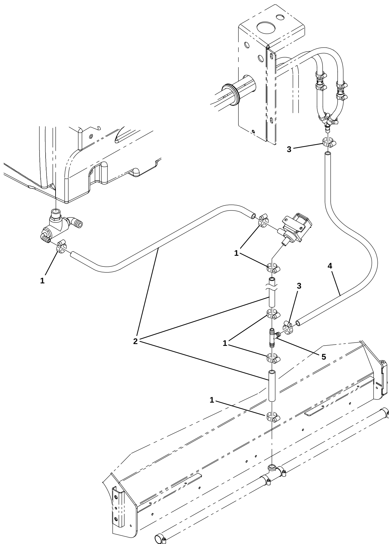
Fig. 17 – FaST Solution Supply Group, Cylindrical Scrub Head (0130– )
