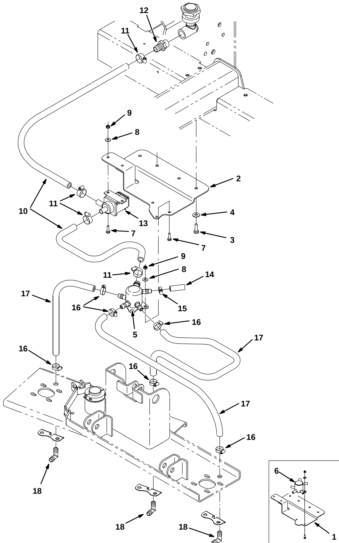
Fig. 45 – Solution Control Group, Disk Scrub Head
