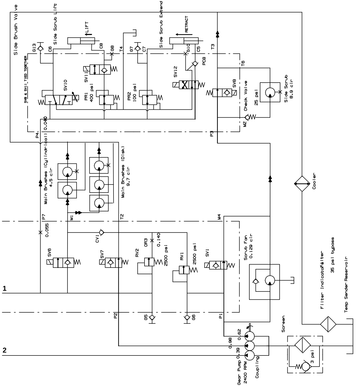
Fig. 51 – Hydraulic Schematic (0245- )
