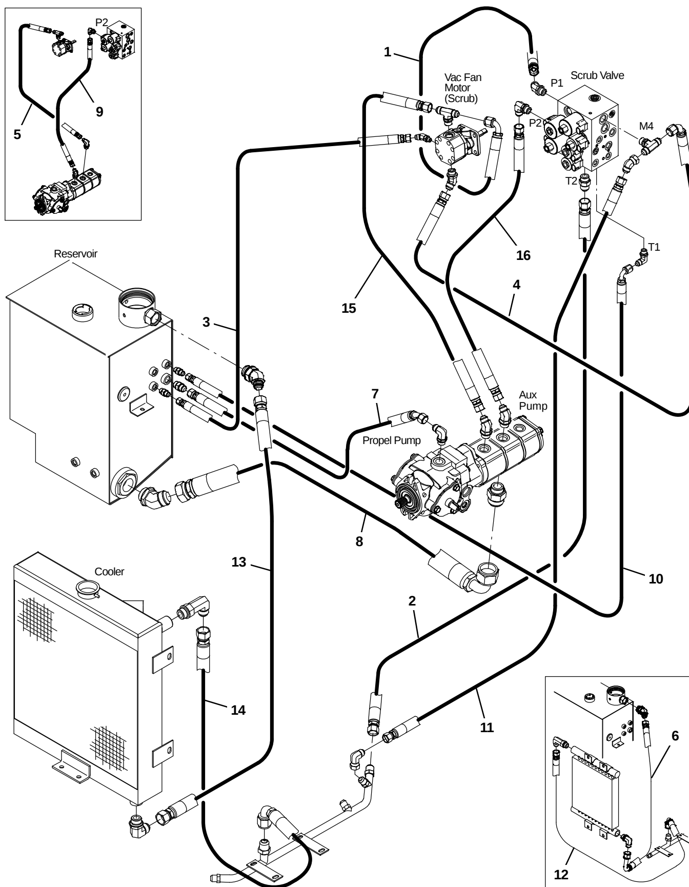
Fig. 53 – Hydraulic Hose Group, Pump and Vacuum Fan
