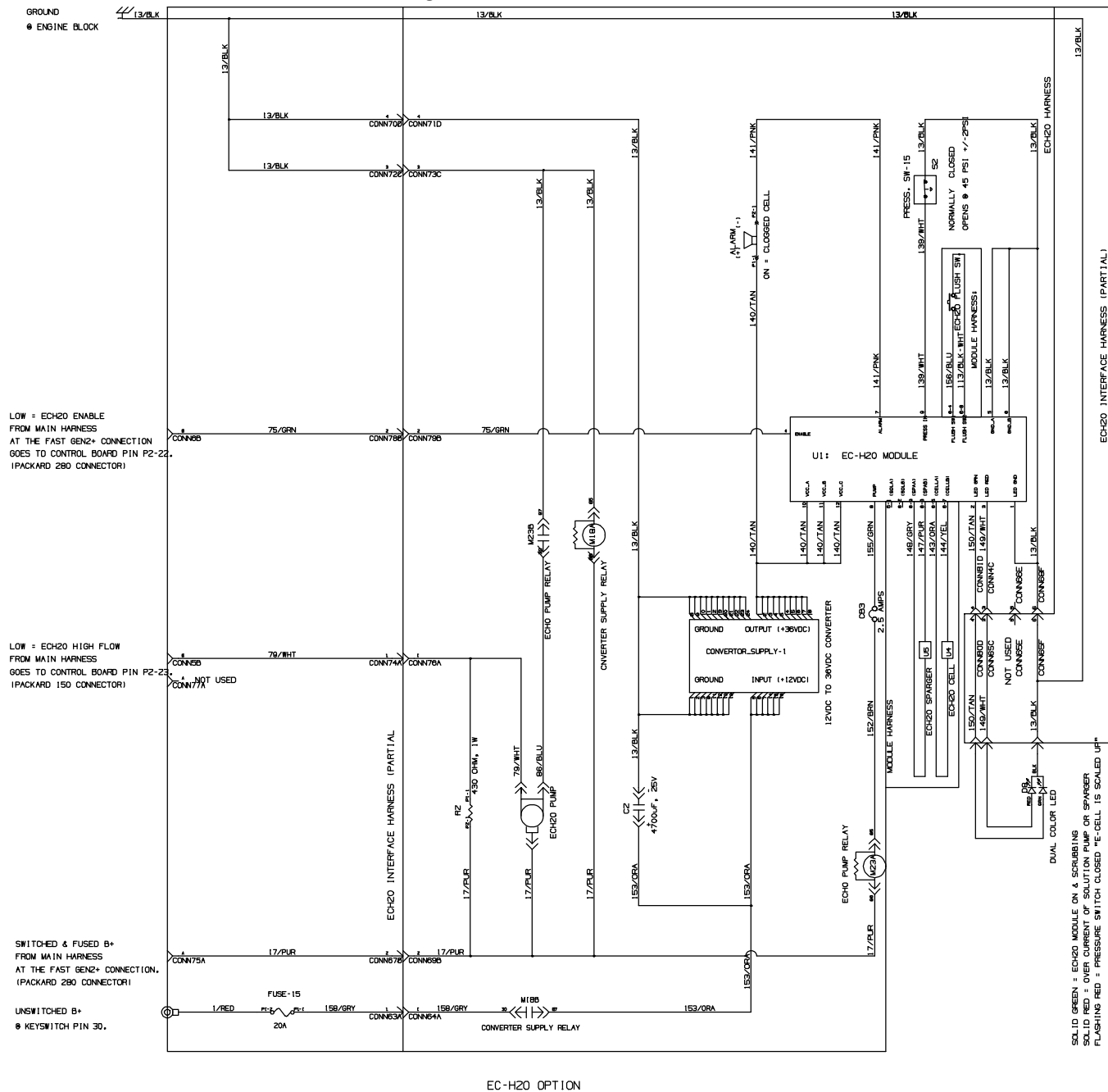
Fig. 61 – Electrical Schematic
