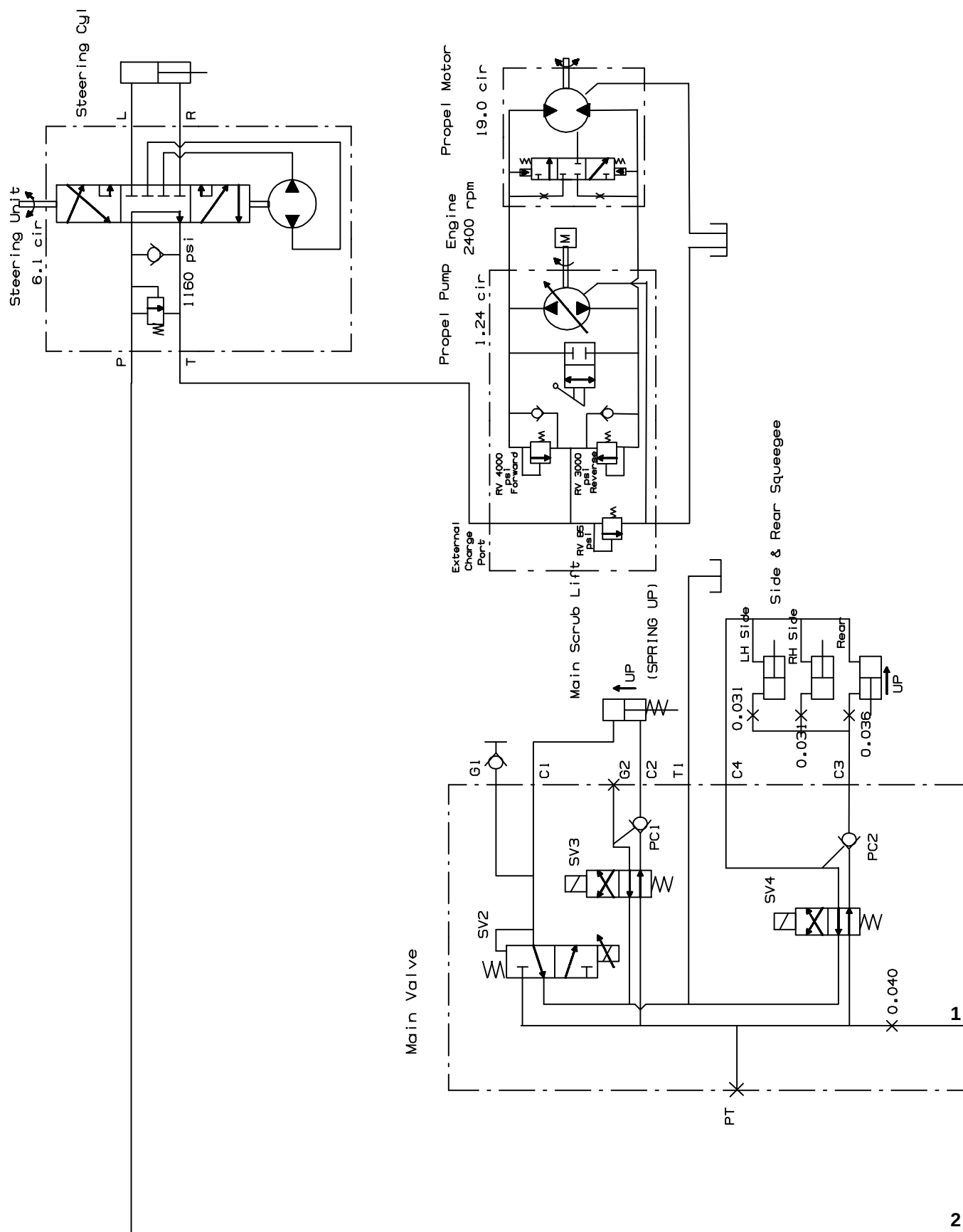
Fig. 51 – Hydraulic Schematic (0245- )
