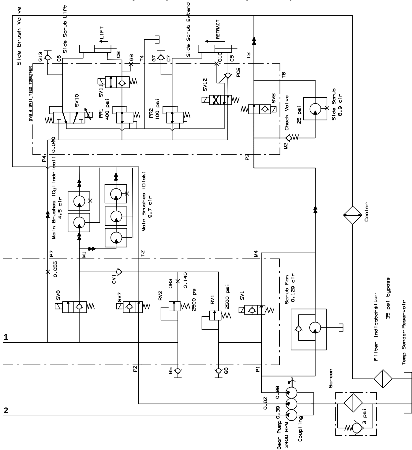
Fig. 50 – Hydraulic Schematic (0043-0244)
