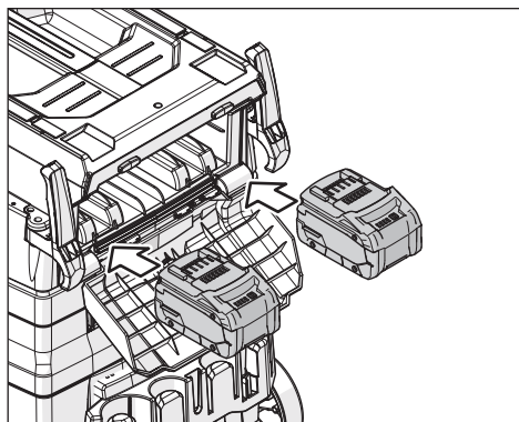
Fig. 10: Battery compartment with two 18 V batteries
