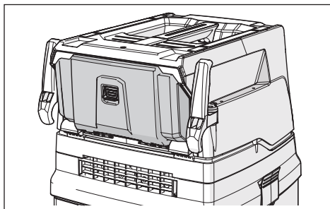
Fig. 9: Battery compartment
