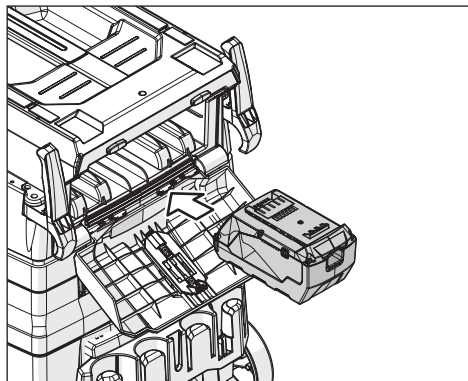
Fig. 11: Battery compartment with a 36 V battery
