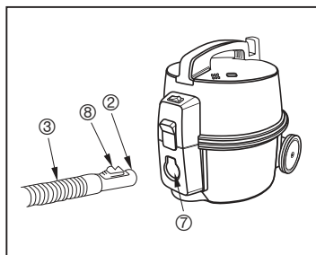
Fig. 3 To attach hose
