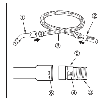
Fig. 2 To assemble hose
