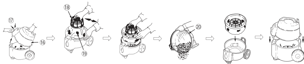
Fig. 12 To remove dust
