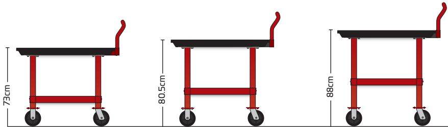
Three height options ranging from 73cm to 88cm with an interval of 7.5cm are available for different work surface heights.
