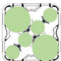
2 Columns: Dia 24.4 to 29.8cm (60 each) 4 Columns: Dia 16.5 to 18.7cm (45 each) Total Capacity: 300
